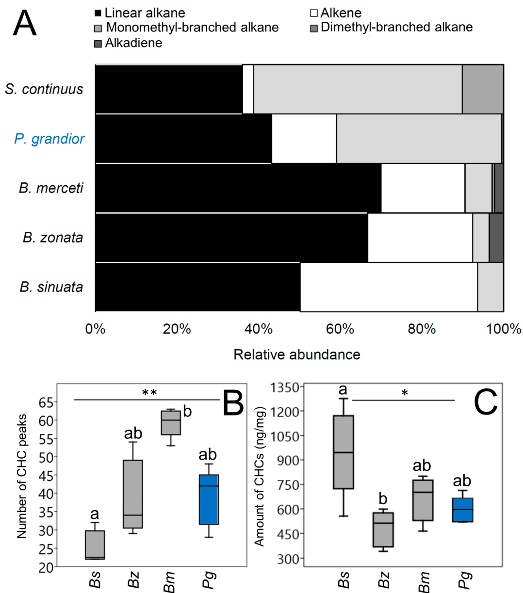
Figure 2. (A) Relative amount (in %) of the hydrocarbons substance classes in the cuticular hydrocarbon (CHC) profiles of P. grandior (in blue), its Bembix hosts and the non-host S. continuus (all in black); (B) Box-and-whisker plots showing medians (horizontal lines within boxes), 1° and 3° quartile (horizontal lines closing the boxes) and maximum and minimum values (ends of the whiskers) for the number of CHC peaks occurring in P. grandior and its Bembix hosts; (C) Box-and-whisker plots showing medians (horizontal lines within boxes), 1° and 3° quartile (horizontal lines closing the boxes) and maximum and minimum values (ends of the whiskers) for the amount of CHCs (nm/mg) on the cuticle of P. grandior and its Bembix hosts. * and ** mean that differences among groups are significant at p < 0.05 and p < 0.01 , respectively; letters identify pairwise differences (Dunn’s procedure). Bs = B. sinuata , Bz = B. zonata , Bm = B. merceti , Pg = P. grandior .
