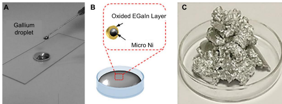
Figure 1. Liquid metal and its mixture. (A) Photo of gallium droplet, reproduced with permission from [69]. (B) Schematic diagram of Ni-GaIn particle, reproduced with permission from [70]. (C) Photo of Cu-GaIn mixture, reproduced with permission from [73].
