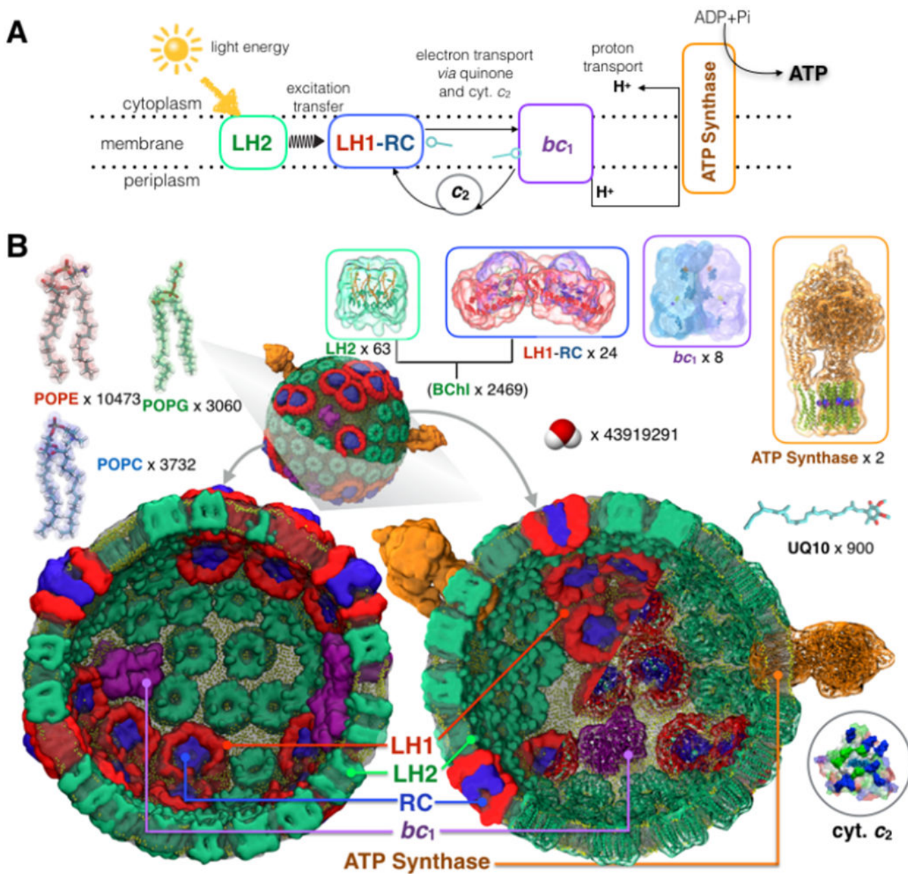
Fig. 1: Physical model of chromatophore.
