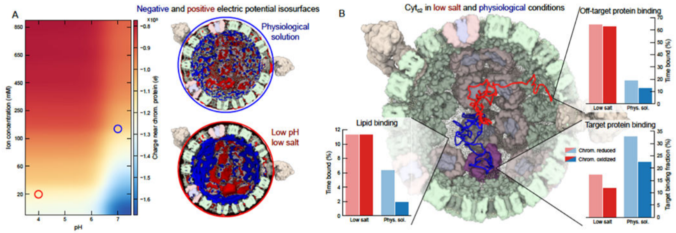
Fig. 5: Phase diagram of chromatophore activity showcases design principles for efficient organelle-scale single-electron transport.
