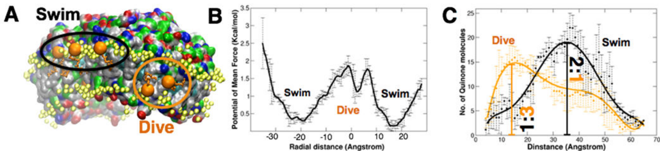
Fig. 4: Dynamics of quinone molecules reveals a two-state model for membrane-mediated charge transport.
