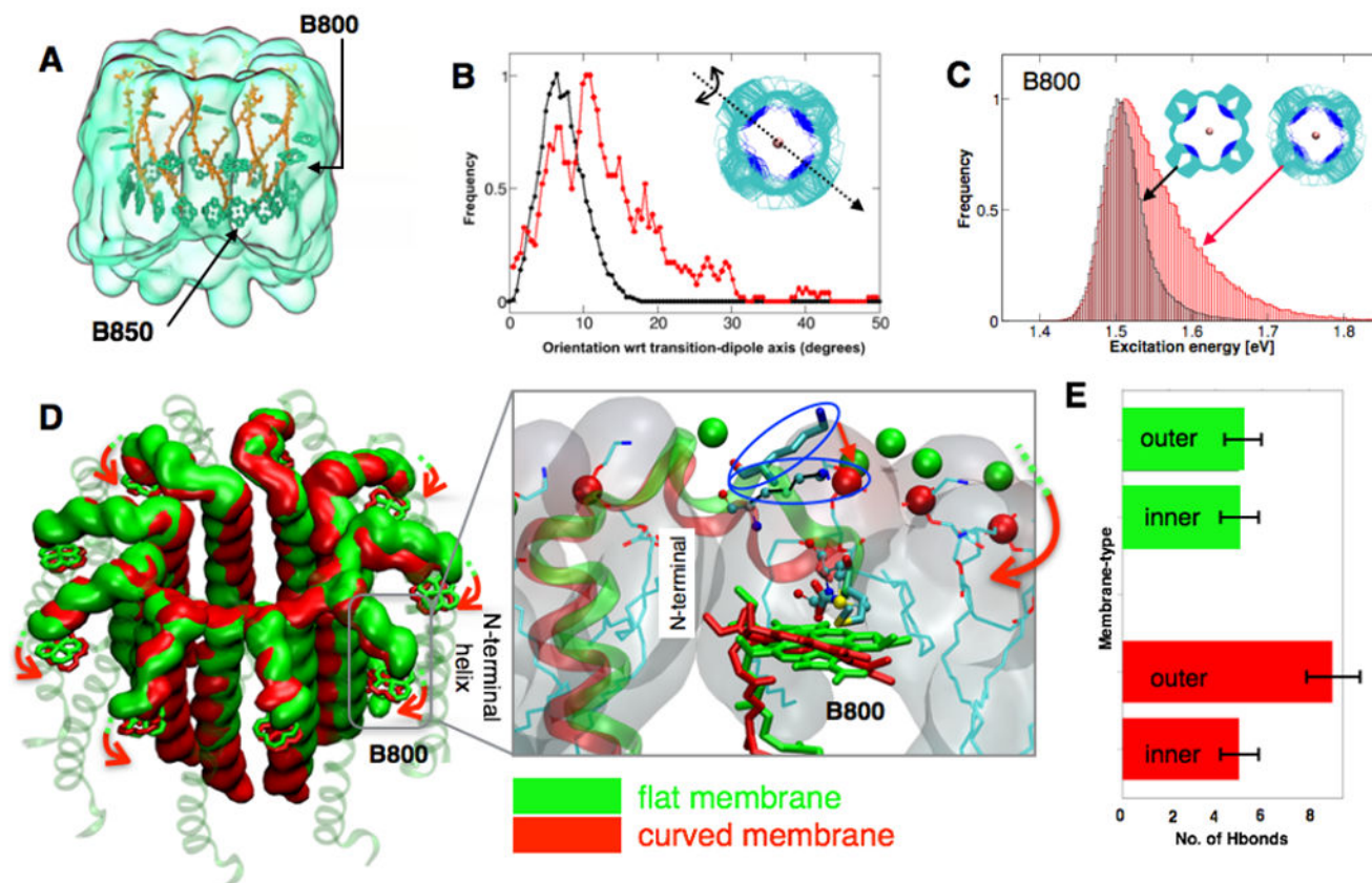
Fig. 3: Thermal disorder in the chromatophore membrane modifies inter-pigment excitation transfer.
