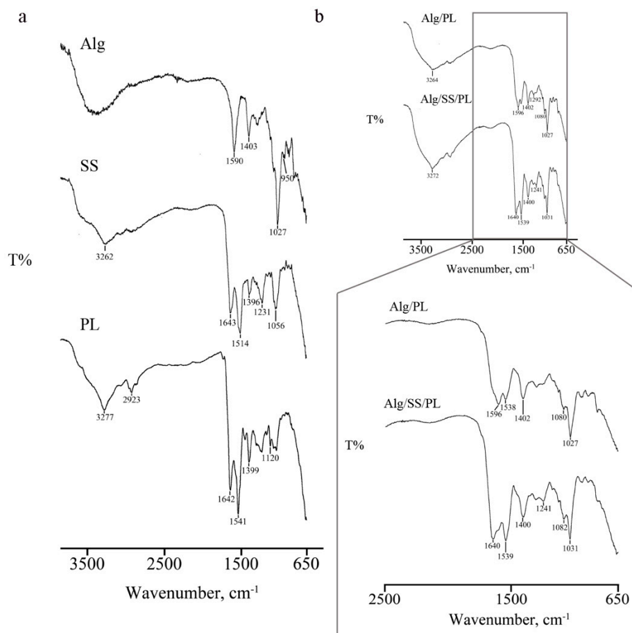
Figure 1. Fourier transform infrared (FTIR) spectroscopy. The analysis was performed on single components (SS, PL and Alg) (a) and biomembranes (b) The IR spectra were obtained in the spectral region of 4000–650 \text{cm}^{-1} .
