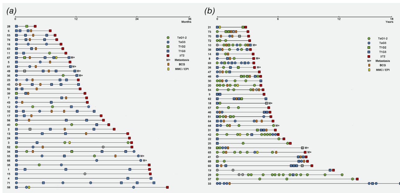
Figure 1. Chronologic disease course for 73 patients with progressive UBC. Patient timelines are shown divided by median time to progression into (a) early progressors with less than 3 years between primary tumor and progression, and (b) late progressors, with more than 3 years to progression. Squares and circles represent tumor manifestations, whereas rectangles represent intravesical treatment courses. Placement of symbols that would overlap due to short time between events has been adjusted minimally. [Color figure can be viewed at wileyonlinelibrary.com ]
