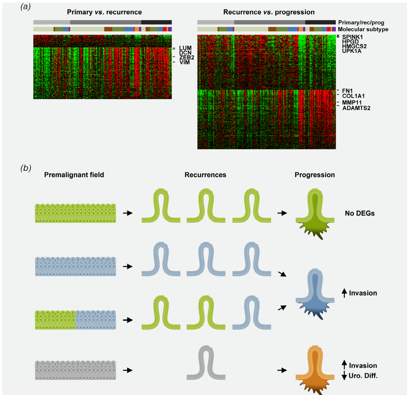
Figure 6. Differential gene expression between primary tumors, recurrences and progression tumors suggests stochastic or punctuated rather than gradual modes of progression. Heatmap in (a) (left) showing expression in the full data set of 135 genes differentially expressed between primary tumors and subsequent recurrences. Genes upregulated in recurrences formed a coherent signature and were mainly coding for ECM components ( LUM , DCN ) and markers of nonepithelial cells ( ZEB2 , VIM ). Heatmap in (a) (right) showing expression in the full data set of 239 genes differentially expressed between the last NMI recurrences and subsequent progression tumors. Genes upregulated in progression tumors formed a coherent signature and were mainly coding for ECM components ( FN1 , COL1A1 ) and genes involved in ECM remodeling and invasion ( MMP11 , ADAMTS2 ). The top downregulated genes in progression tumors were members of a urothelial differentiation signature expressed in luminal-like subtypes ( SPINK1 , HPGD , HMGCS2 and UPK1A ). Ordering by molecular subtype, revealed such downregulation primarily in nonluminal-like tumors and the same analysis, limited to patients with stable Urothelial-like subtype (UroA, light green, UroB, brown or UroC, dark green) resulted in no significant DEGs. (b) Schematic model suggesting different modes of progression in bladder cancer: In the stable modality (first and second panels), patients recur and progress stably within the Uro subtype (green color) or the GU subtype (blue color), suggesting a common origin of all recurrences in a premalignant field that only produces tumors of one subtype. In the unstable modality (third and fourth panels), patients either develop both Uro or GU recurrences and progress with a GU subtype, or progress to a nonluminal-like subtype (orange color, bottom). Patients that progress with a nonluminal-like subtype had few prior recurrences that could be of any subtype (gray). The unstable modality of progression involves radical shifts in molecular subtype over the disease course suggesting an underlying premalignant field that is either heterogeneous or evolving to give rise to various subtypes. [Color figure can be viewed at wileyonlinelibrary.com ]
