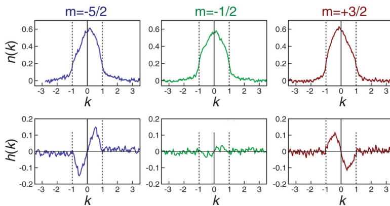
FIG. 17. Direct visualization of an edge-state current for a two-dimension (one real, one synthetic) lattice in the presence of an artificial magnetic field. Upper row: Momentum distributions n_m(k) along the real direction x for the three values of the pseudospin m corresponding to the synthetic direction. The value m = -1/2 can be viewed as the bulk, whereas m = +3/2 and m = -5/2 corresponding to the opposite edges of the sample along the synthetic dimension. Lower row: Function h_m(k) = n_m(k) - n_m(-k) . From Mancini et al. , 2015.
