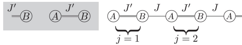
FIG. 30. A semi-infinite SSH model. The left region (gray area) has J=0 , hence a winding number N=0 . The right region may have N=0 or 1, depending on the ratio J/J' . In the latter case a zero-energy edge state resides close to the boundary between the two domains.
