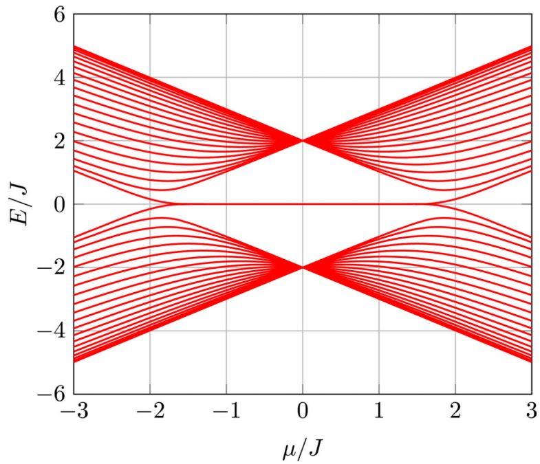
FIG. 34. Quasiparticle spectrum of \hat{H} - \mu\hat{N} [Eq. (A8)] for an open chain of 20 sites and t = J . The pair of solutions (E, -E) with E \approx 0 that appears in the topological region |\mu| < 2J represents the Majorana zero energy modes at the two ends of the chain.
