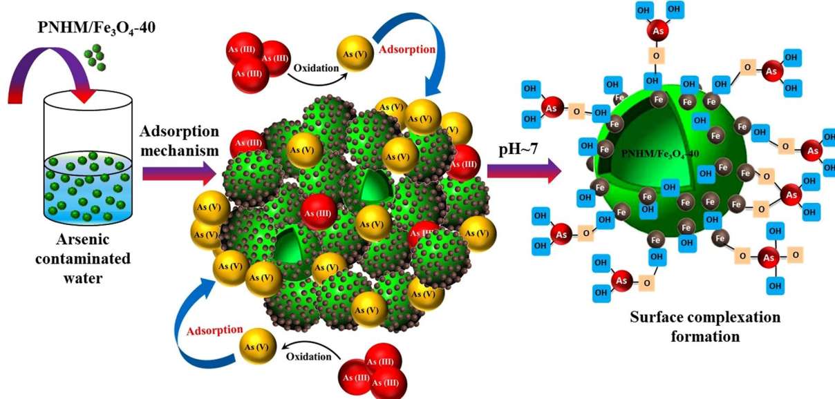
Figure 7. Schematic representation of arsenic adsorption mechanism in aqueous solution.
