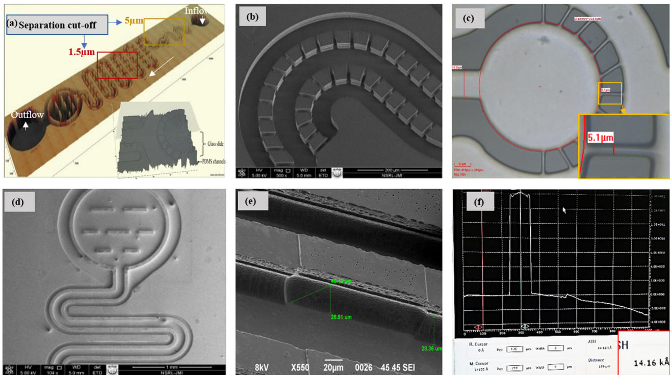
FIG. 4. Microscopic images of filter arrangement of the device: (a) 3D image of the complete device, (b) array of pillar filters (width 5.5\text{--}6\mu\text{m} and 30\mu\text{m} height) arranged in the t-flow mode, (c) particle collection reservoir with pillar microfilters arranged in the n-flow mode, (d) t-flow arrangement of weir filters ( 1.5\text{--}2\mu\text{m} ) bound via a dead-end weir filter, (e) tilted image of a single weir filter, and (f) height of weir as 1.42\mu\text{m} measured using a stylus profiler.
