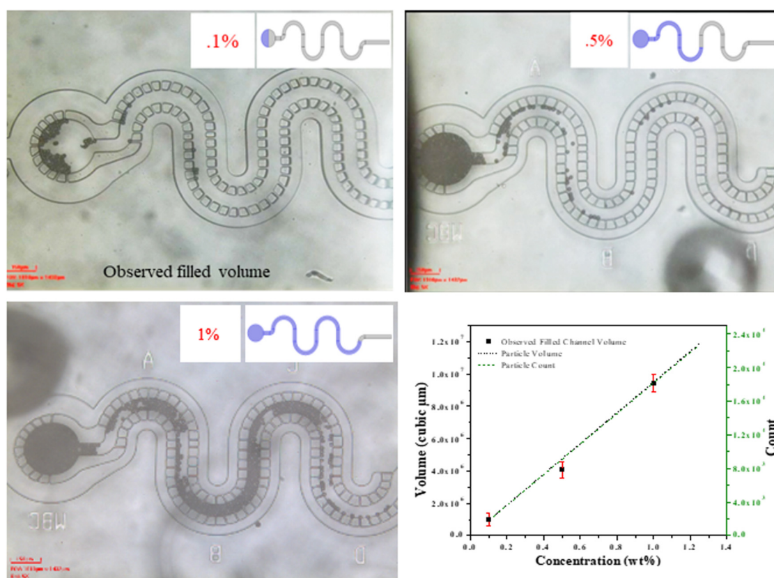
FIG. 8. Particle concentration and channel volume filling comparison obtained by 10 \mu\text{m} monodisperse particle suspension. Analytically calculated volume and count of microparticles for given concentration are compared with experimentally obtained filled microchannel volume with equivalent particle concentrations.
