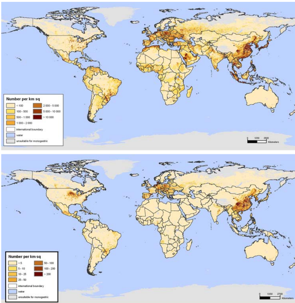
Figure 2. Global poultry (top) and swine (bottom) distributions (FAO, 2007).
