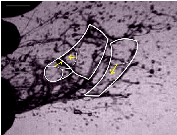
Fig. 7 Example of multiple sneeze-induced expanding sheets after rupture. The image is shown at 22 ms after the sneeze began. Video SIV1 in the electronic supplementary materials shows the full sequence. Scale bar is 1 cm. We provide the associated video SIV1 in the electronic supplementary materials
