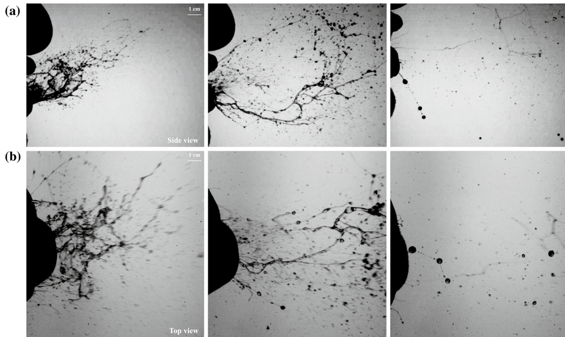
Fig. 6 Stages of sneeze ejecta imaged from a the side and b the top, respectively. The first column features the initial sheet and bag bursting after 8 ms. The second column shows the ligament formation, elongation, and pearl formation at 21 ms, and the third column
