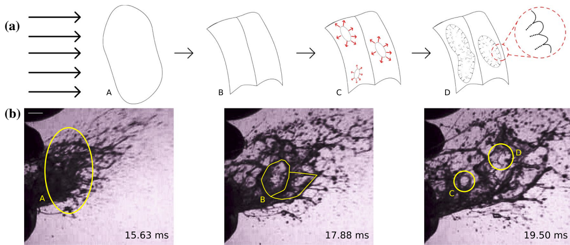
Fig. 1 a Schematic of the fragmentation process of a liquid volume in response to applied aerodynamic forces and b photographs recorded shortly after the first appearance of sneeze ejecta. The initial liquid volume ( A ) is flattened into a sheet ( B ), followed by hole for-
