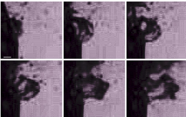
Fig. 8 Development of the bag instability at the edge of the lip. The bag first grows into a mucus bubble then deforms prior to finally bursting. The snapshots are shown at intervals of 0.5 ms. The bag was originally nearly spherical in shape. This sequence was recorded at 8000 fps. Scale bar is 2 mm
