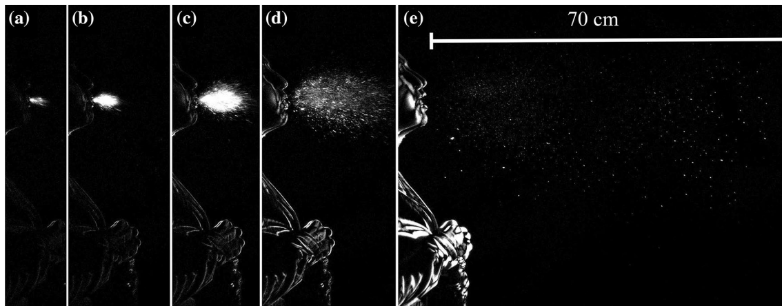
Fig. 3 Cough recorded with high-speed imaging at 1000 fps and displayed at a 0.005, b 0.008, c 0.015, d 0.032, and e 0.15 s from onset
