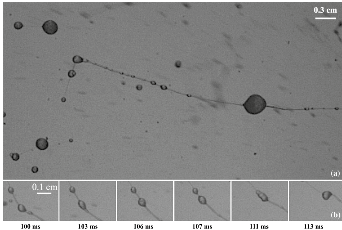
Fig. 10 Beads on a string. a Multiscale droplets or “pearls” form on stretching ligaments owing to the influence of non-Newtonian effects. This snapshot is taken 130 ms after the onset of the sneeze and is
