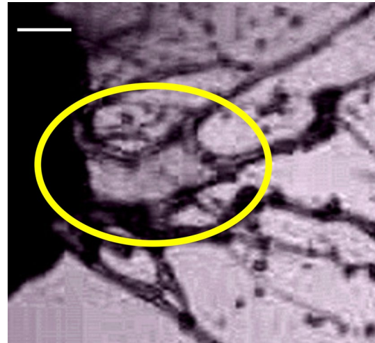
Fig. 9 Bag shown here (highlighted by the oval) originates from the mouth near the lower lip. It is in the form of a flattened sheet of horizontal extent of approximately 16 mm. This image was captured at 40 ms from the onset of a sneeze. Scale bar is 5 mm
