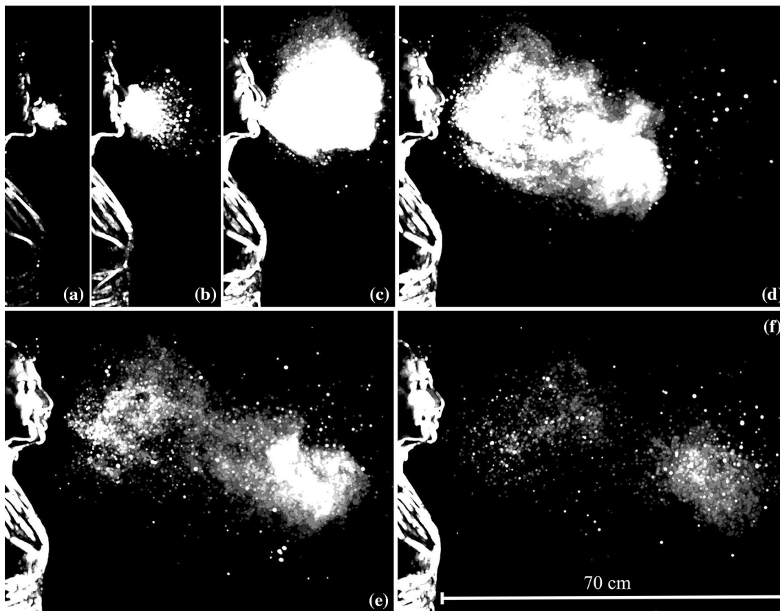
Fig. 4 High-speed images recorded at 1000 fps for a sneeze at times a 0.007, b 0.03, c 0.107, d 0.162, e 0.251, and f 0.34 s. The multiphase sneeze cloud grows by turbulent entrainment as it advances
