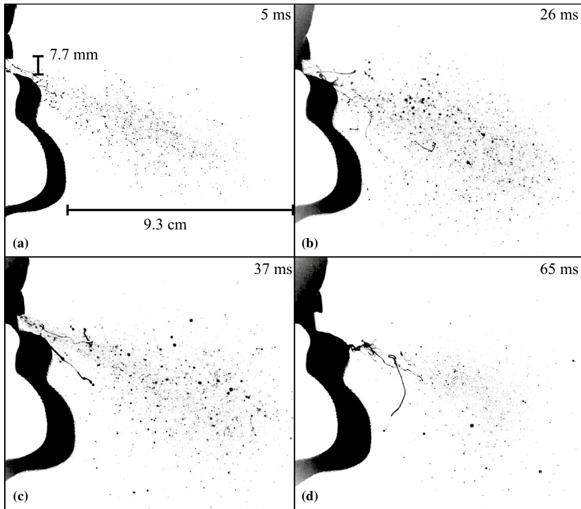
Fig. 5 Sequence of sneeze emissions at a 5, b 26, c 37, and d 65 ms after the onset of a sneeze. The sequence is recorded at 2000 fps using diffused backlighting. The mouth diameter was approximately 8 mm. The motion of the head throughout the sneeze is highlighted
