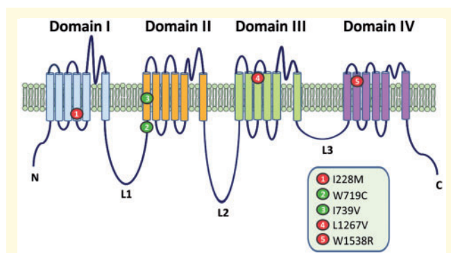
Figure 2 Topology of the human Na v 1.7 sodium channel, with the location of I228M, W719C, I739V, L1267V and W1538R. All but one mutation (W719C) are located in the VSDs of the channel. The two lacosamide-responsive mutations are shown in green. Both are located within the vicinity of Domain II: W719C is located at the end of Linker I and I739V in VSD II. Non-responsive mutations are indicated in red. All three variants (I228M, L1267V and W1538R) map to the VSD in Domains I, III and IV, respectively.
