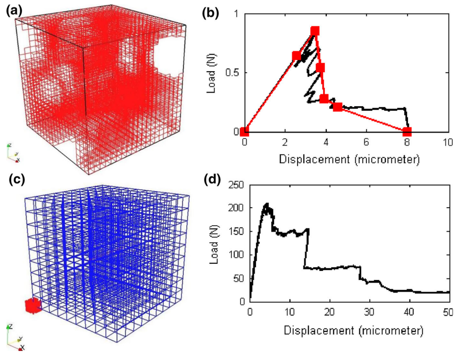
Fig. 3 Multi-scale modelling procedure: a a small cube, 20 \times 20 \times 20 voxels; b load-displacement curve (black), which is the outcome of a small-scale simulation. The red curve is a schematisation of the black one and is a multi-linear curve with six segments with points taken at (1) origin; (2) first micro-cracks; (3) peak load; (4) first point in response for which load is <75\% of
