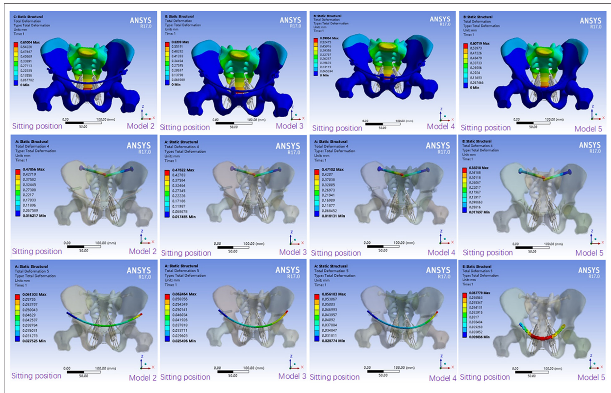
Figure 4. Displacement distribution of fixed models in sitting position.
