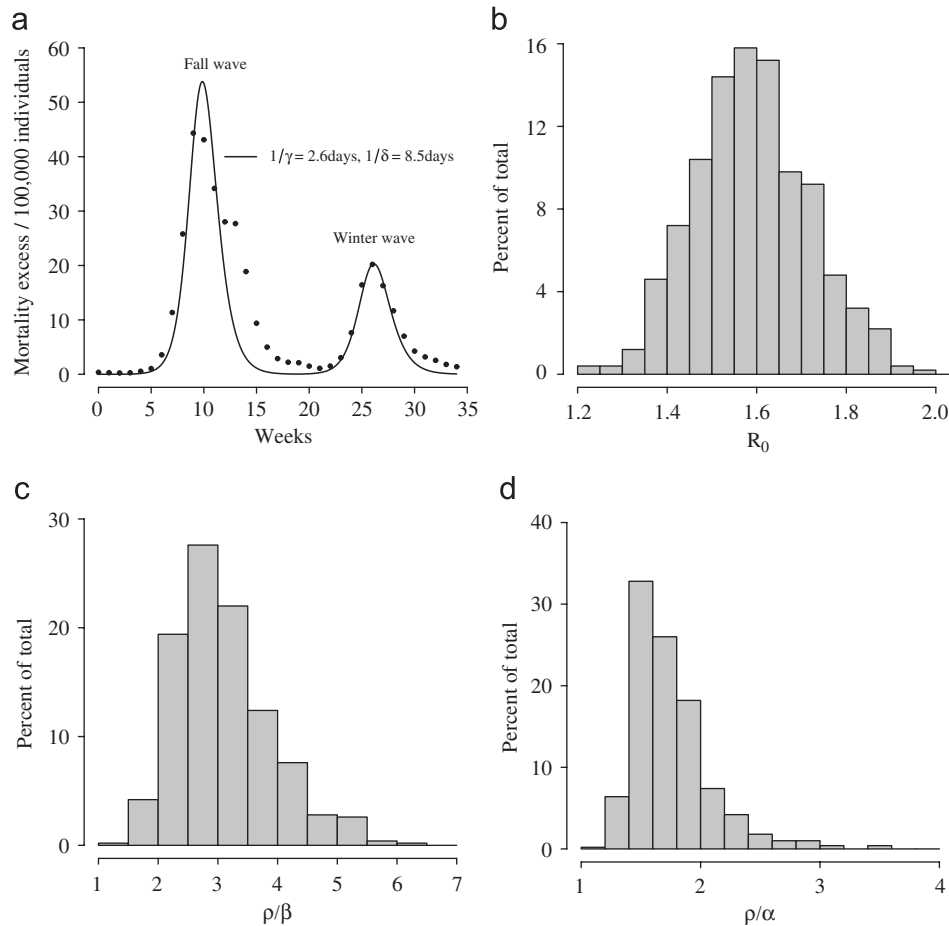
Fig. 4. (a) The best-fit solution obtained by fitting model (1) to the GB data (filled circles, initial time 24 August 1918). (b) Distribution of R_0 . (c) Distribution of \rho/\beta . (d) Distribution of \rho/\alpha .
