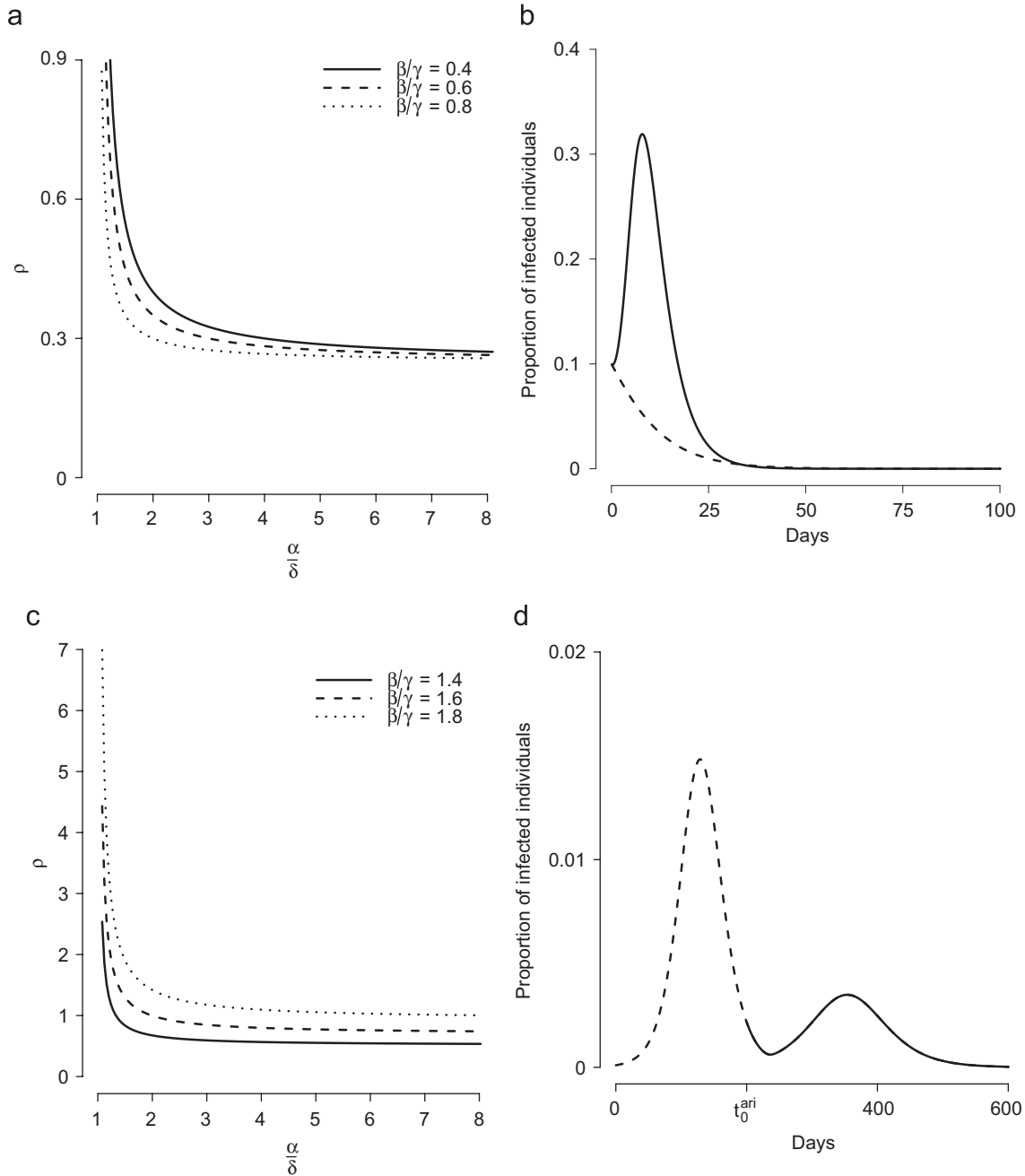
Fig. 2. (a) Threshold value \rho(R_0^{\text{ari}}) for different values of \beta/\gamma (keeping fixed \gamma = 0.25 ) and S^* = 1 . (b) For S^* = 1 , \beta = 0.2 and \gamma = 0.25 , dashed line represents the proportion of infected individuals in the absence of ARI, while solid line represents the proportion of infected individuals in presence of ARI ( \alpha = 1, \delta = 0.25, \rho = 0.8, t_0 = t_0^{\text{ari}} = 0 ). (c) As in (a) but for S^* < 1 (at the end of the first epidemic wave). (d) For S^* < 1 , dashed line represents the proportion of infected individuals before the onset of ARI, while solid line represents the proportion of infected individuals after the onset of ARI. Parameters employed: \beta = 0.3, \gamma = 0.25, \alpha = 1, \delta = 0.25, \rho = 0.8, t_0 = 0 and t_0^{\text{ari}} = 200 .
