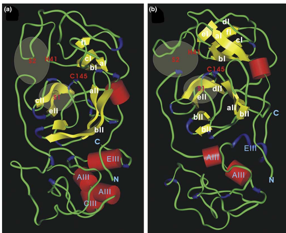
Fig. 2. The homology model of (a) M pro ST and (b) M pro SH visualized by Insight II. \alpha -Helices and \beta -strands are shown in red cylinders and yellow arrows, respectively. The general acid–base catalyst His residue and the nucleophilic Cys residue are labeled. The locations of the putative substrate binding subsites S1 and S2 are indicated.
