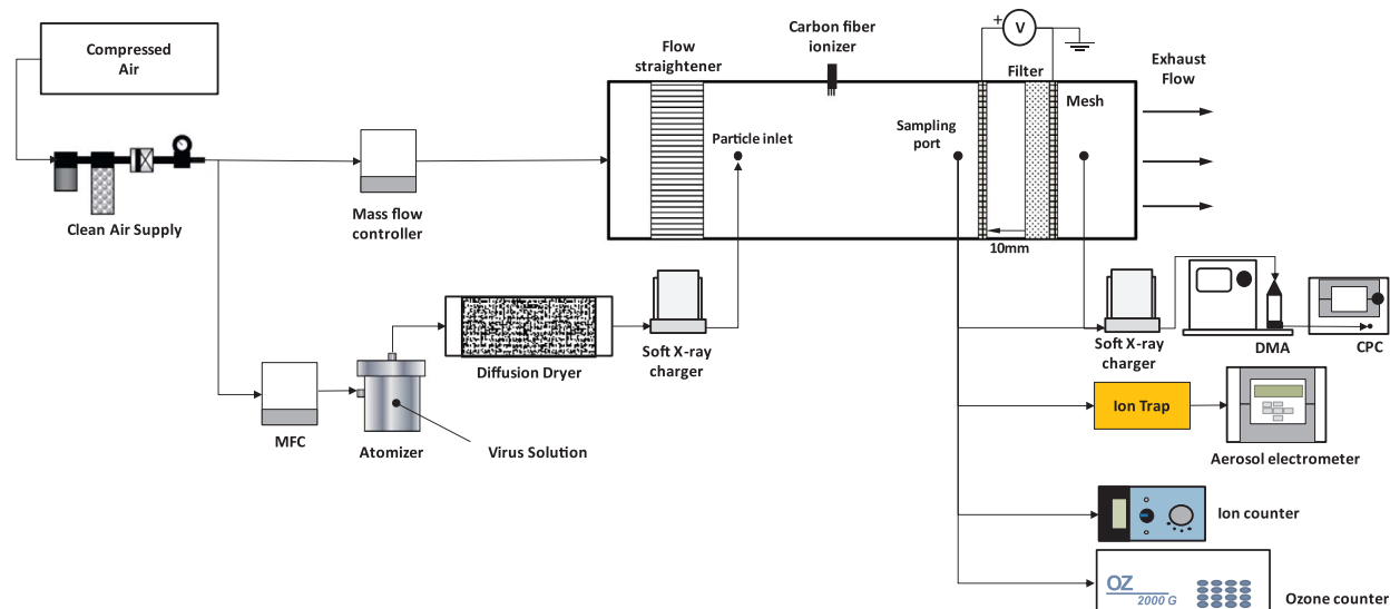
Fig. 1. Experimental setup.
