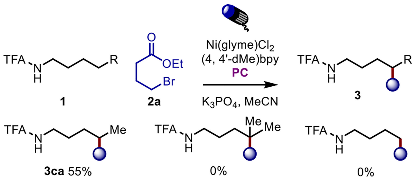
Scheme 2. Effect of Substitution at \delta -position.
