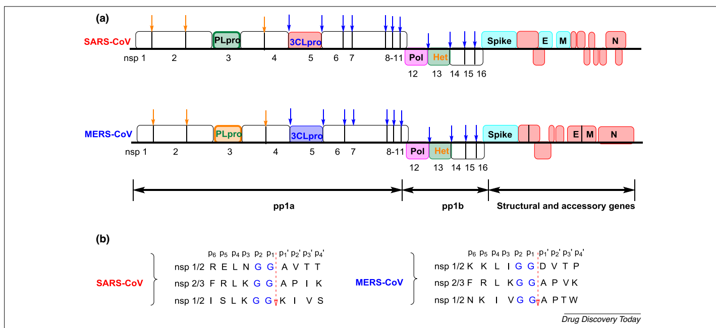
FIGURE 6 Overview of SARS and MERS-CoVs polyproteins. (A) Cleavage positions of PL pro and 3CL pro are shown by arrows. (B) Cleavage site comparison between SARS and MERS PL pro enzymes (For SARS-PL pro : (L/I)XGG↓(A/D)X and for MERS-PL pro : LXGG↓(A/K)X).
