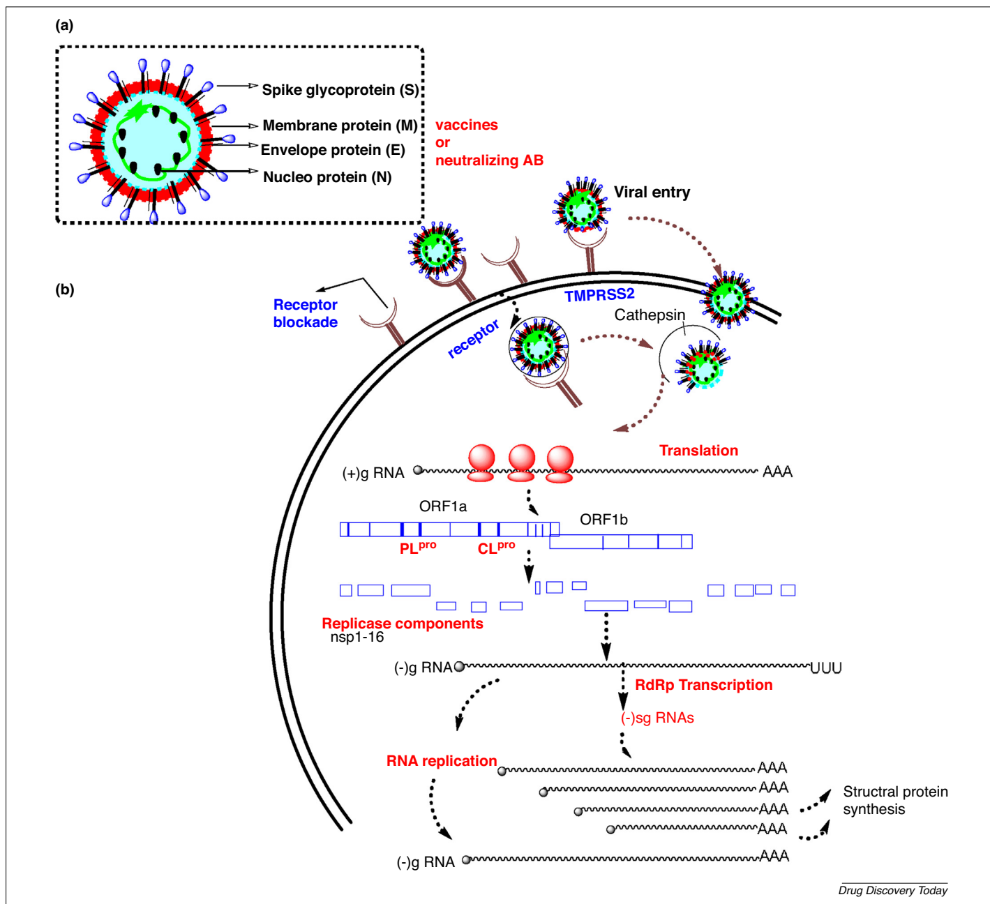
FIGURE 2 (A) Structure of coronavirus and (B) its replication: (Ab: Antibody; DPP4: Dipeptidase Peptidyl 4; TMPRSS2: Transmembrane Protease, Serine 2; PL pro : Papain-like Protease; 3CL pro : 3-C-like Protease; RdRp: RNA dependent and RNA polymerase; nsp: Non-structural protein, ORF: open reading frame, ACE2: Angiotensin converting enzyme, CD13: human aminopeptidase N). Entry targets: (I) Spike protein (RBD, Fusion intermediates); (II) Receptors; a. DPP4/CD26 for MERS, b. ACE2 for SARS and HCoV-NL63, c. 9-O-Acetylated sialic acid for HCoV-OC43 and HCoV-HU1, d. CD13 for HCoV-229E (III) Surface proteases: TMPRSS2. (IV) Endosomal proteases. Polyprotein processing targets: a. Papain-like protease (PL pro ), b. 3C-like protease (3CL pro ). Replicase targets: a. ADP-ribose-1'-phosphatase (nsp3), b. RNA-dependent and RNA polymerase (nsp12), c. Helicase (nsp13), d. Exonuclease (nsp14), e. Endoribonuclease (nsp15), f. 2'-O-methyltransferase.
