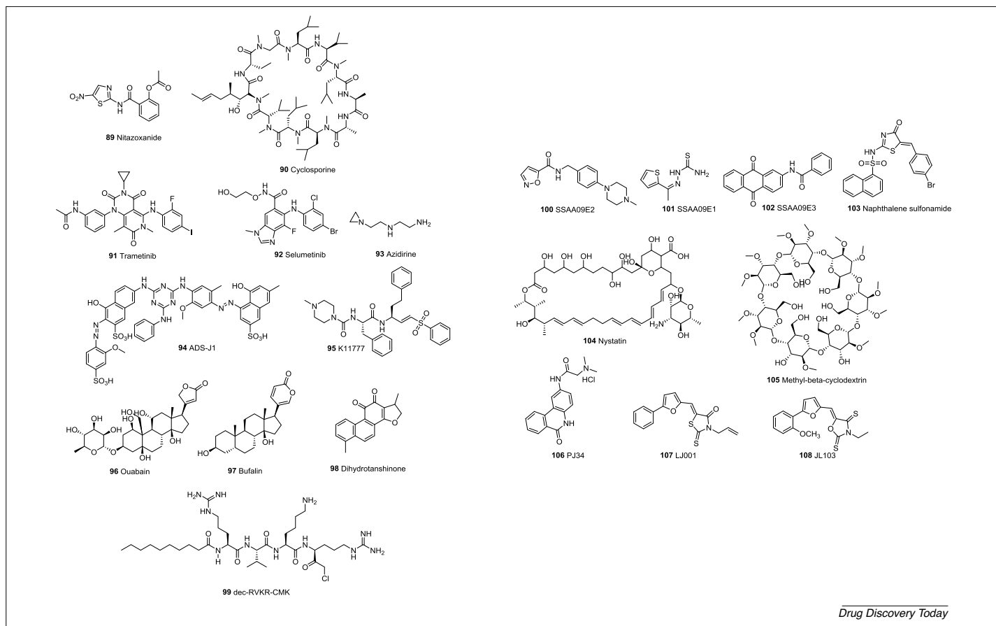
FIGURE 13 Representative host-based anti-Coviral drugs for CoV infections.
