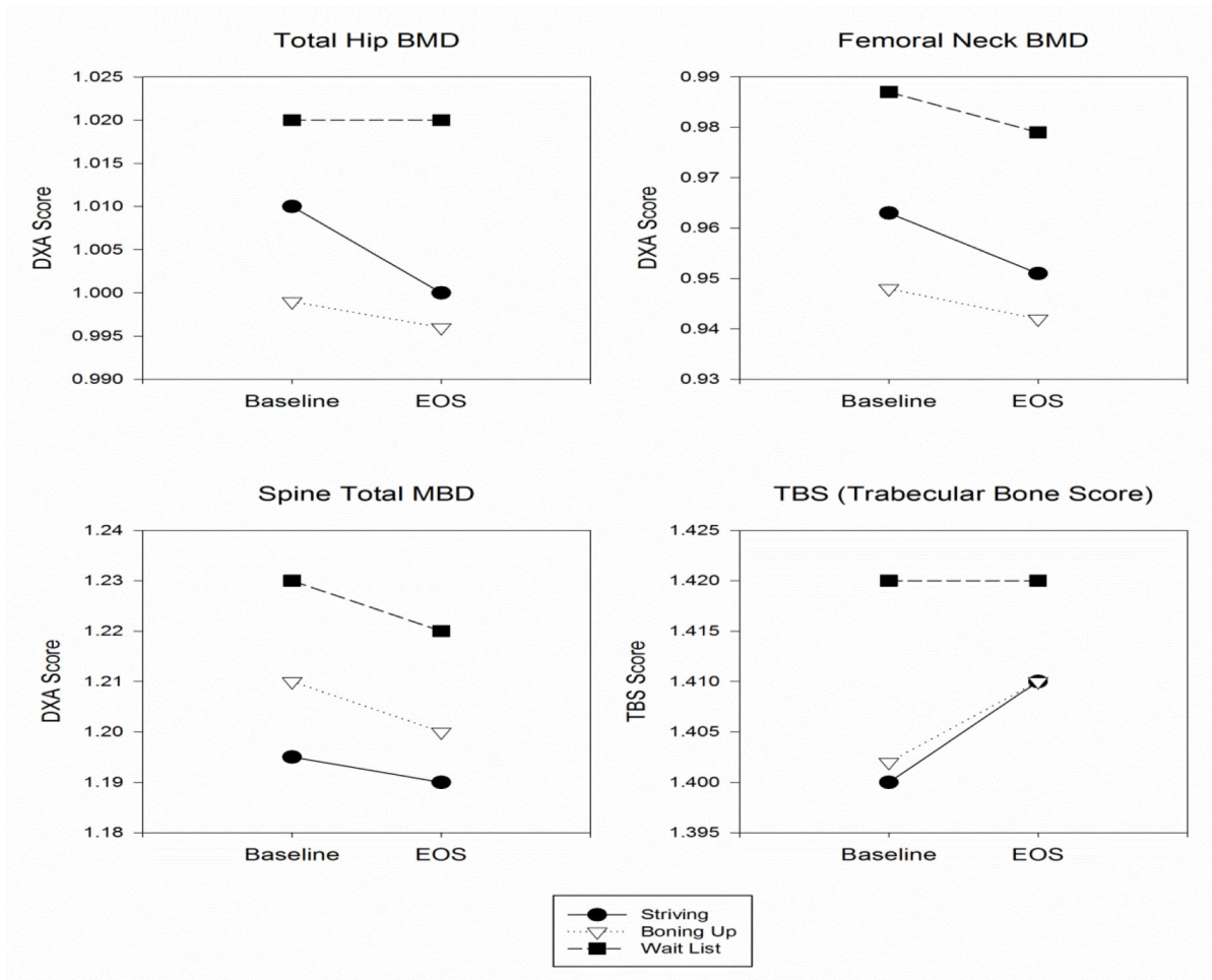
Figure 2: Graphic Representation of Change in Bone Mineral Density and Trabecular Bone Score over Time and Among Groups The downward slopes of the lines depict loss of bone mineral density & trabecular bone score between baseline and end of study for total hip, femoral neck, and spine. No difference among the groups occurred as evidenced by none of the lines crossing over time.
