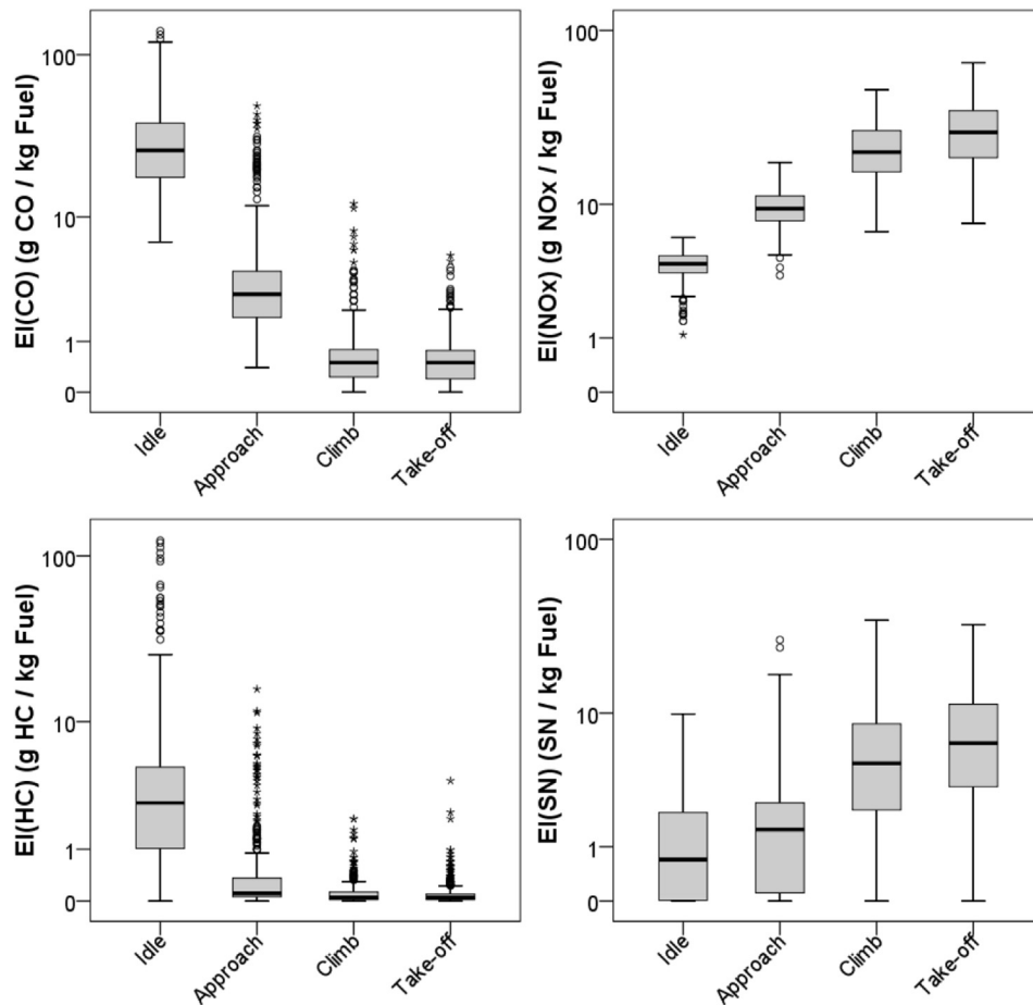
Fig. 7. EIs provided by the ICAO databank (EASA, 2013). All in-use engines certified from 1976 to today (April 2013) are included.
