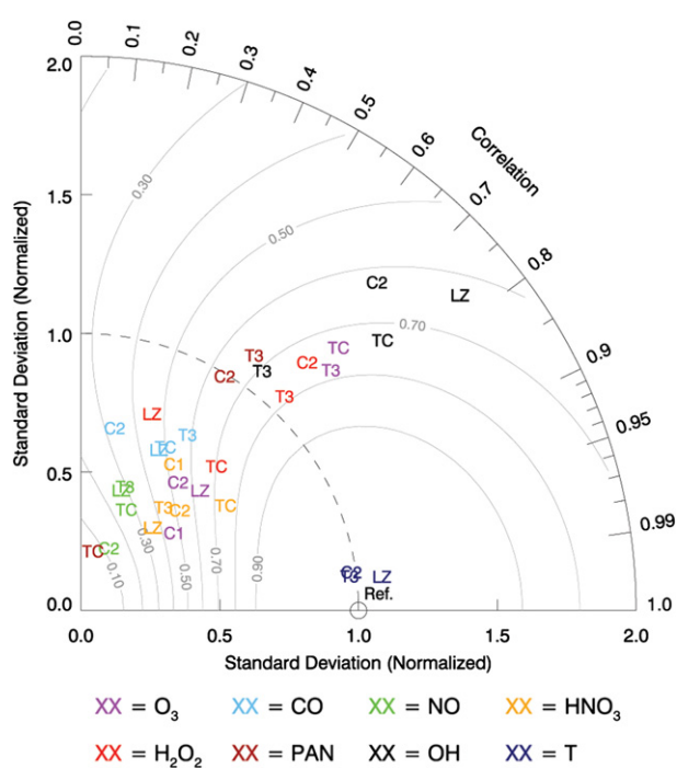
Fig. 11. Taylor diagram for 4 models: TM3(T3), OsloCTM2 (C2), TOMCAT (TC), and LMDz/INCA(LZ) applied in the TRADEOFF project in a comparison of model output for various species with measurements made between 1995 and 1998 in an altitude range between 5.5 km and 13 km over the North Atlantic (adapted from Brunner et al., 2003).
