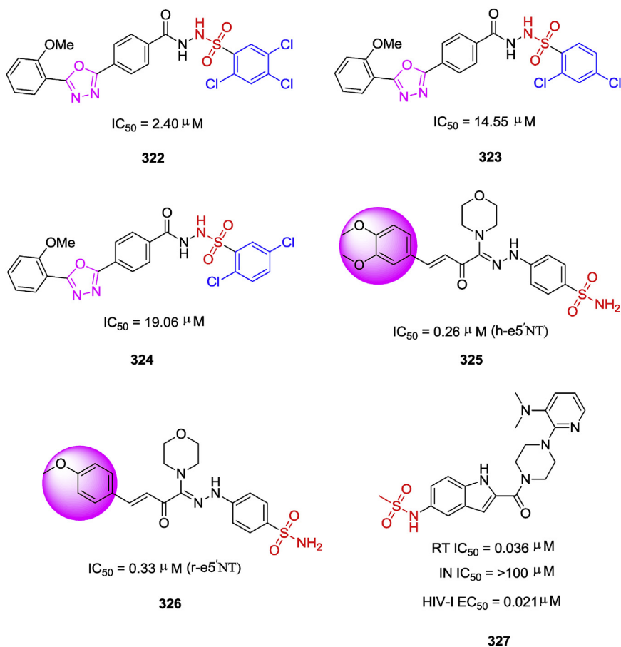
Fig. 40. Sulfonamide or sulfonamides with diverse pharmacological properties.
