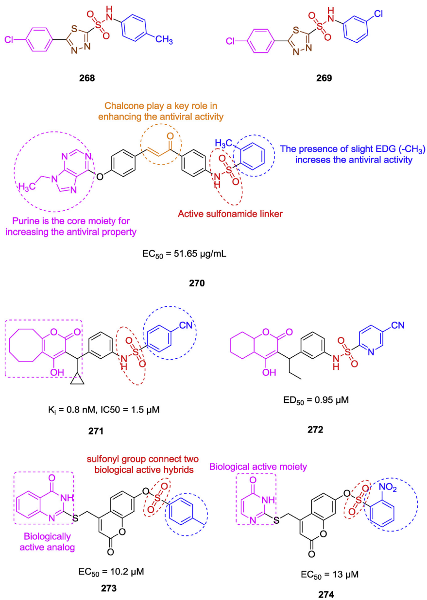
Fig. 32. Sulfonyl or sulfonamides potent anti-viral agents.
