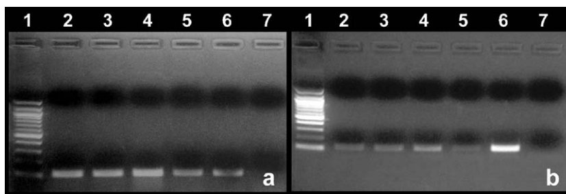
Fig. 7. FECV-specific RT-PCR on clinical samples from ferrets with ECE. (a) Lane 1, 100-bp DNA ladder. Lanes 2–5, amplicons from fecal specimens collected from one of the ferrets on days 0, 7, 12, and 26, respectively. Lane 6, FECV positive control (113-bp product). Lane 7, negative reagent control (RNase-free water as the template). (b) Lane 1, 100-bp DNA ladder. Lanes 2–5, amplicons from saliva specimens collected from one of the ferrets on days 0, 7, 12, and 26, respectively. Lane 6, FECV positive control (113-bp product). Lane 7, negative reagent control (RNase-free water as the template).
