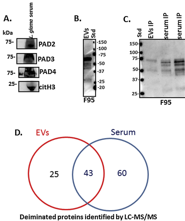
Fig. 2. Western blotting of deiminated proteins and PAD in llama serum. A. Llama PAD homologues were identified at the expected size of approximately 70–75 kDa using the anti-human PAD2, PAD3 and PAD4 isozyme specific antibodies respectively. Deiminated histone H3 (citH3), representative of neutrophil extracellular traps (NETs), was verified in llama serum. B. Total deiminated proteins were assessed by Western blotting in llama serum EVs, using the F95 pan-deimination specific antibody. C. Immunoprecipitated (IP) deiminated proteins after F95-enrichment were assessed both in serum-EVs and whole serum of llama by Western blotting. D. The Venn diagram represents deiminated proteins identified in total serum and serum-derived EVs by F95 enrichment and LC-MS/MS analysis. Overall, 43 proteins were identified in common with both samples, while 60 proteins were found deiminated in serum only and 25 proteins were identified as deiminated in EVs only.
