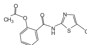
Fig. 1. Chemical structures of nitazoxanide, tizoxanide and RM-5038.
