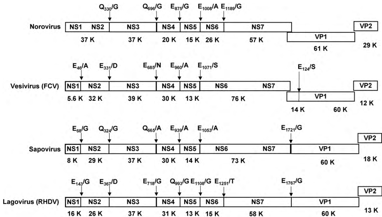
Fig. 3. Comparison of the organization of the viral genome of the six calicivirus genera. The complete genome of the following strains is shown: Norovirus GII.4 (Hu/NLV/Dresden174/pUS-NorII/1997/GE strain, GenBank accession no. AY741811), vesivirus (feline calicivirus, FCV/Dresden/2006/GE strain, GenBank accession No. DQ424892), sapovirus GI.1 (Hu/SV/pJG-Sapl/DE strain, GenBank accession no. AY694184), and lagovirus (RHDV strain RHDV/Dresden/2006/GE, GenBank accession no. EF363035). The cleavage sites in the viral polyprotein precursor are indicated, as well as the putative molecular weight in kDa (K) of the resulting non-structural proteins.
