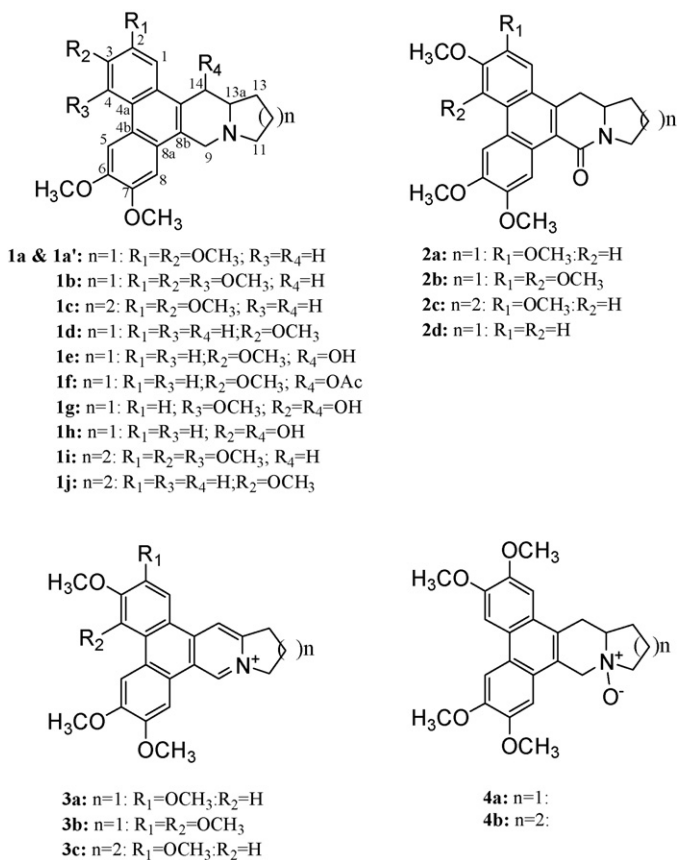
Fig. 1. Chemical structures of phenanthroindolizidine and phenanthroquinolizidine compounds. Phenanthroindolizidines, 1a ( 1a' ), 1b , 1d–1h , 2a , 2b , 2d , 3a , 3b , and 4a , consist of the moieties of phenanthrene and indolizidine and phenanthroquinolizidines, 1c , 1i , 1j , 2c , 3c , and 4b of phenanthrene and quinolizidine. These phenanthroindolizidines and phenanthroquinolizidines are tri-, tetra-, or penta-methoxylated at C2, C3, C4, C6, or C7 in the moiety of phenanthrene and with or without hydroxylated or OAc- at C14, formation of C9-one, or N-oxide in the indolizidine/quinolizidine moiety as shown.
