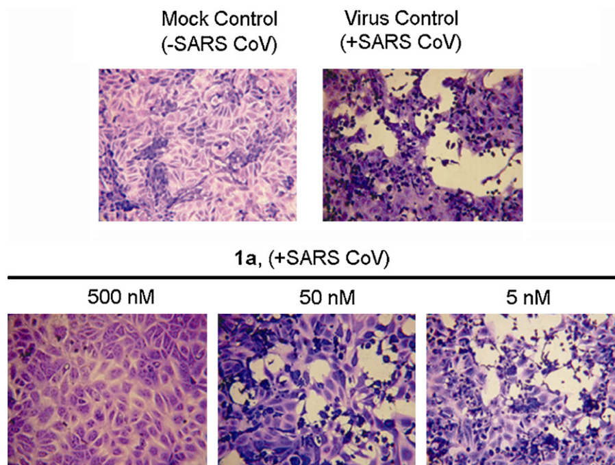
Fig. 4. Anti-SARS CoV activity of tylophorine. SARS CoV and the indicated concentrations of tylophorine ( 1a ) were added in equal volumes to near-confluent cell monolayers of Vero 76 cells in culture plates. The MOI used was ranged from 0.01 to 0.025 to produce virus cytopathic effects in 100% of the cells in the virus control wells within 3–4 days along with a mock infection control. The plates were incubated at 37 °C until the cells in the virus control wells showed complete viral CPE as observed by light microscopy and stained with neutral red as described (Barnard et al., 2006). Equal field areas of each treatment were shown from microscopic observation at 100× magnification.
