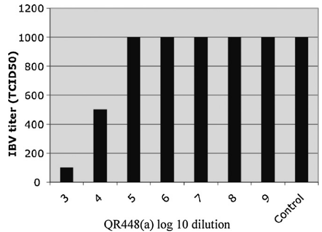
Fig. 1. Titration of IBV Beaudette strain in Vero E6 cells following treatment with 10-fold serial dilutions of QR448(a) starting at 1 \times 10^{-3} to 1 \times 10^{-9} in cell culture maintenance medium and cell culture maintenance medium plus IBV alone (control) are presented. The 50% tissue culture infectious dose (TCID 50 ) titers reflect the average of three replicates. No reduction in virus titer was observed for IBV treated with the diluent (data not shown).
