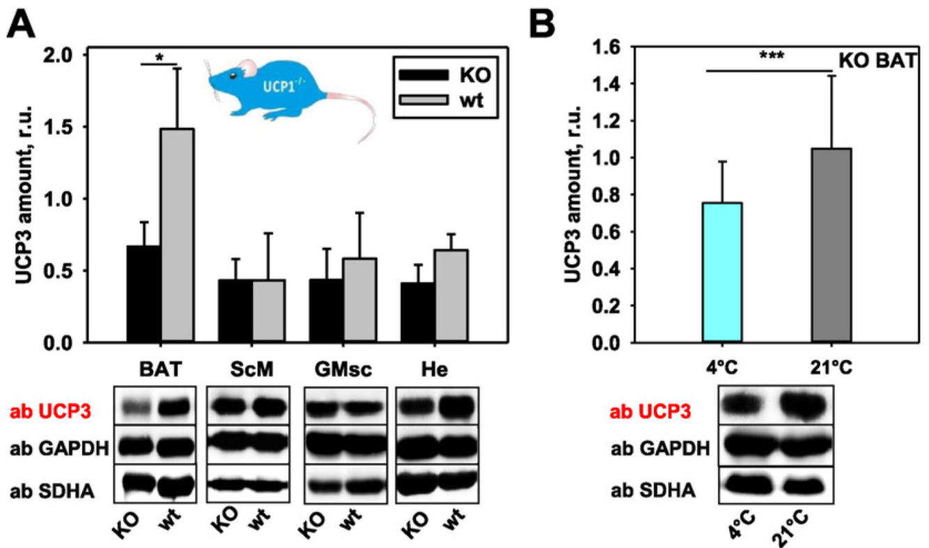
Fig. 4. Representative Western blots and quantification showing UCP3 expression in UCP1^{-/-} mice.
