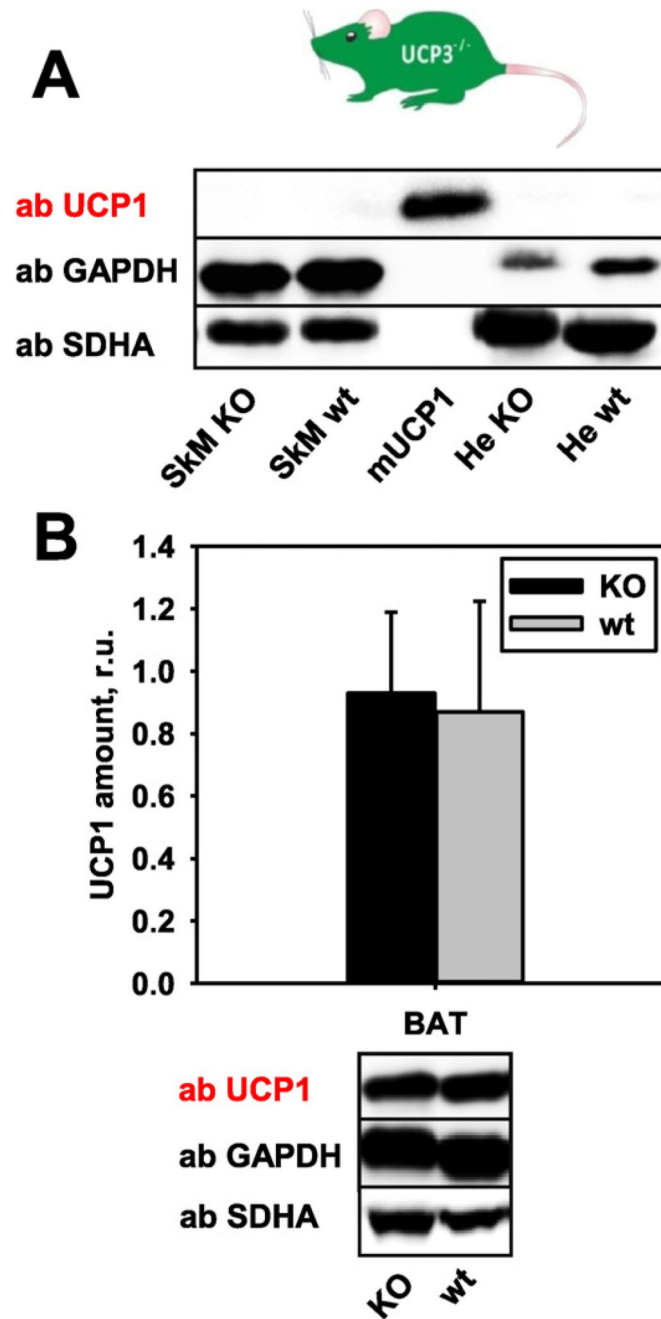
Fig. 5. Representative Western blots and quantification showing UCP1 expression in UCP3 -/- mice.
