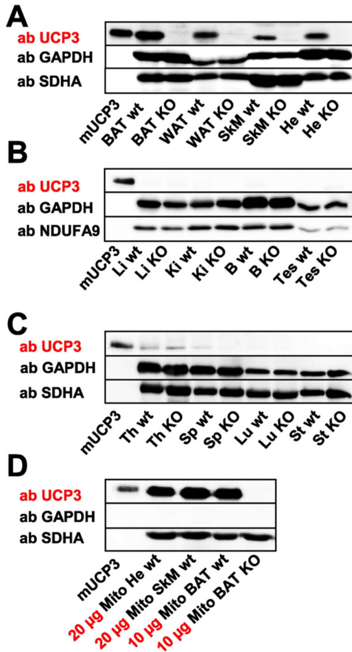
Fig. 1. UCP3 expression patterns in murine tissues under physiological conditions. (A) UCP3 was detected in skeletal muscle (SkM), heart (He), brown adipose tissue (BAT) and white adipose tissue (WAT) of wild type (wt) mice. Corresponding tissues from UCP3 -/- mice were used as a negative control. (B–C) Kidney (Ki), liver (Li), brain (B), testes (Tes), thymus (Th), spleen (Sp), lung (Lu) and stomach (St) show no detectable UCP3 expression. 25 µg of total protein from the tissue were loaded per lane. Five mice per group were tested. (D) UCP3 expression in isolated mitochondria. 20 µg isolated mitochondria from He, SkM and 10 µg isolated mitochondria from BAT were loaded per lane.
