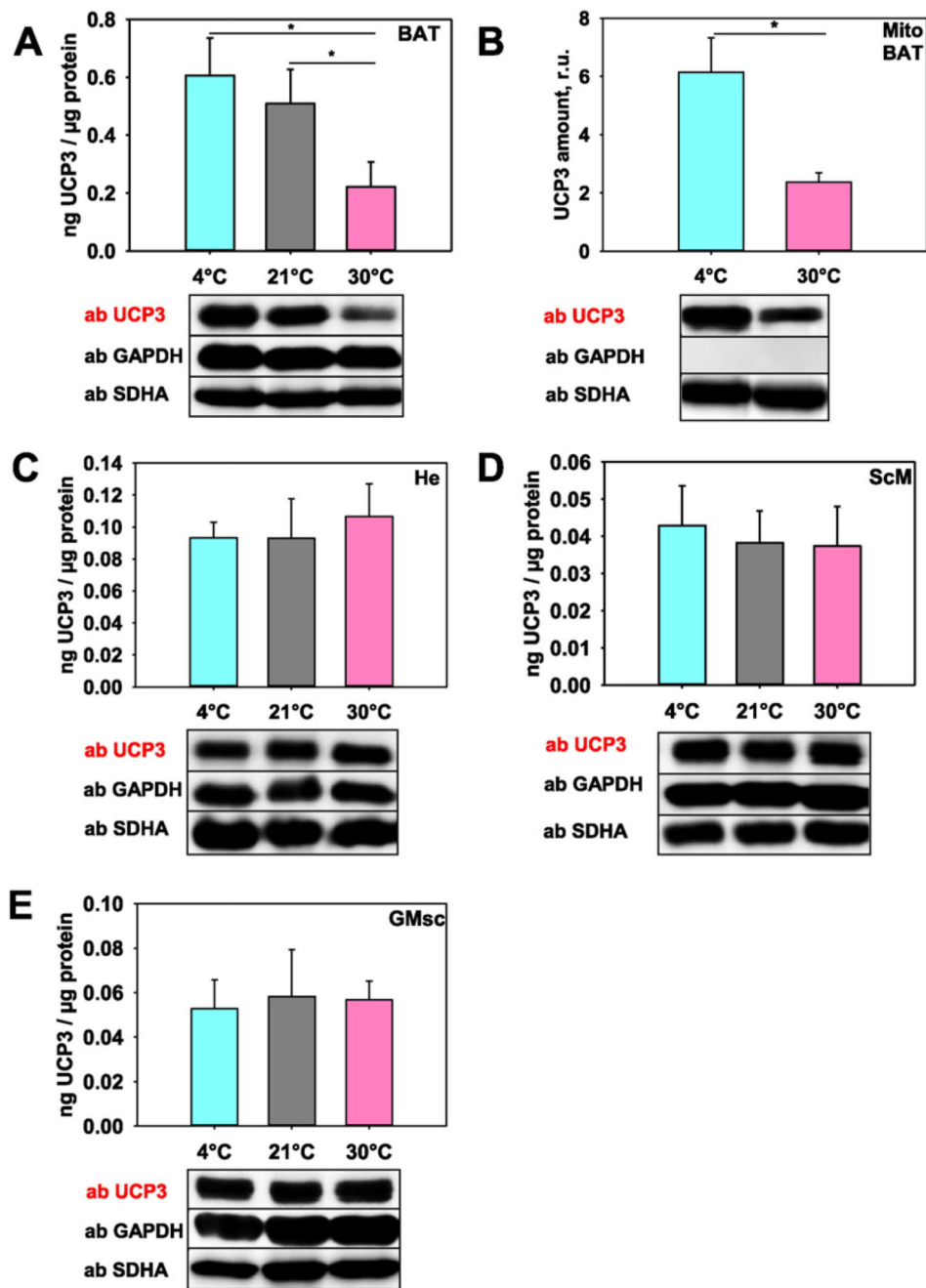
Fig. 3. Quantification of UCP3 expression at different temperatures.
