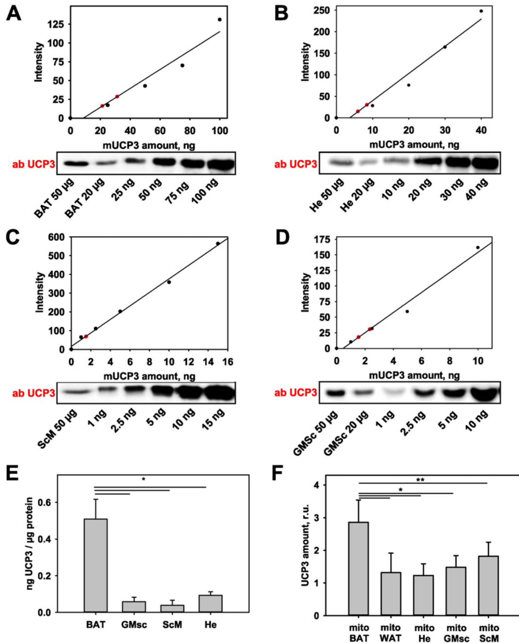
Fig. 2. Protein quantification in tissues expressing UCP3.
