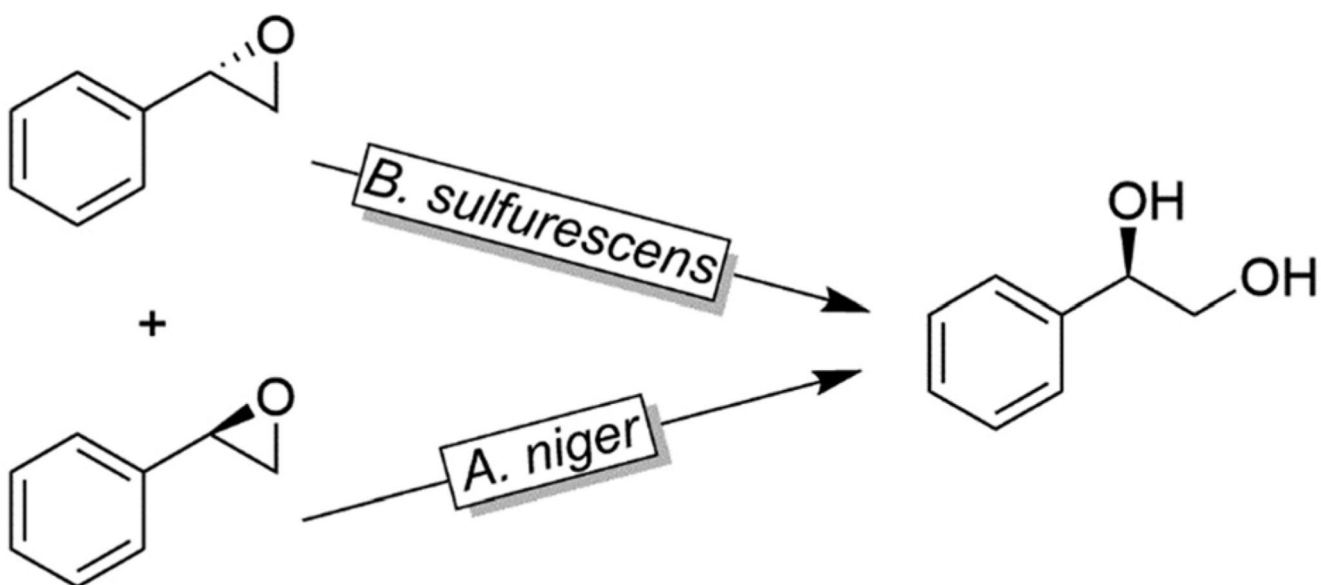
Scheme 32.
