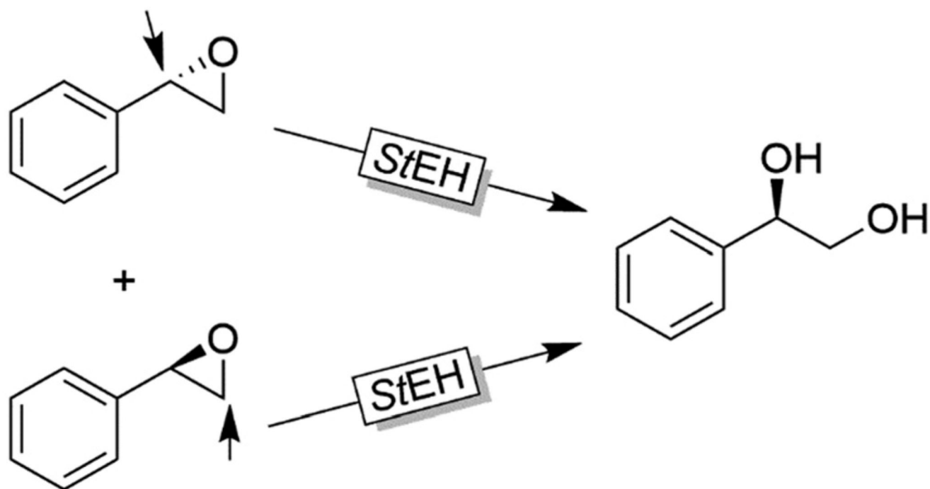
Scheme 33.
