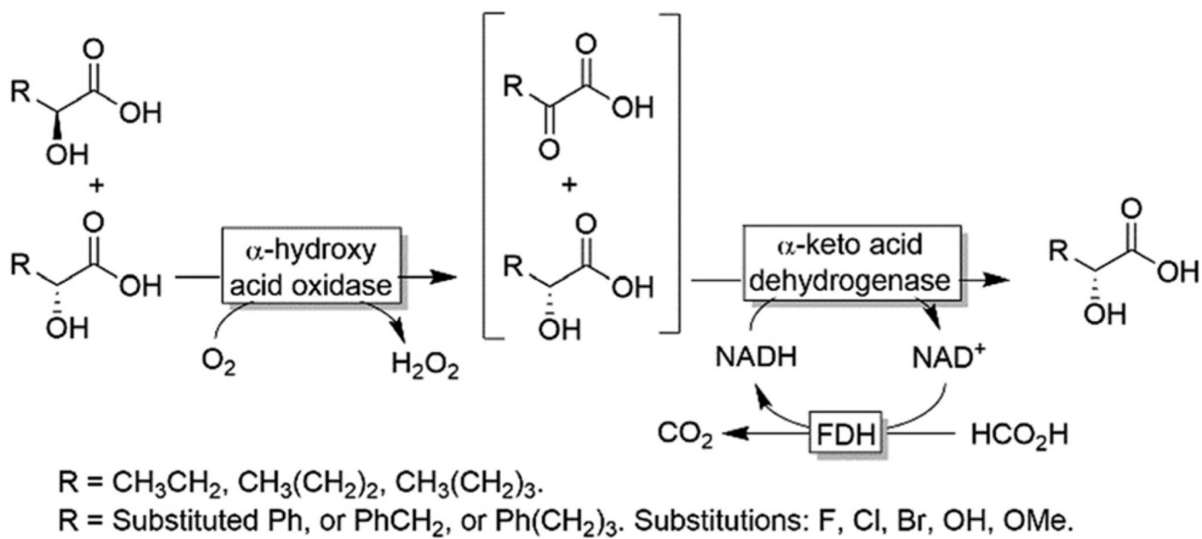
Scheme 15.
