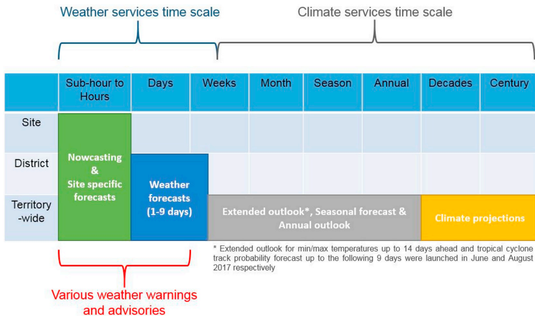
Fig. 3. Spatial and temporal coverage of weather and climate services in Hong Kong.
