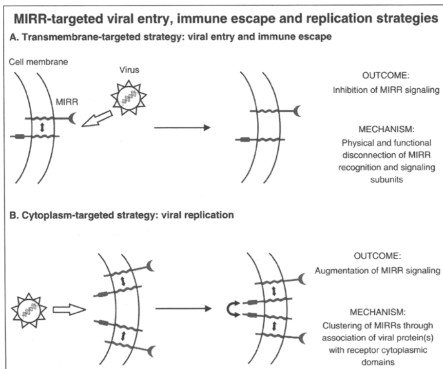
Figure 1. Targeting MIRR: suggested immunomodulatory strategies used by viruses to entry target cells, survive and replicate. Transmembrane interactions between MIRR recognition and signaling subunits are shown by black arrows. Immunoreceptor tyrosine-based activation motifs (ITAMs) are shown as gray rectangles. Circular arrow indicates viral agent-induced receptor clustering.
