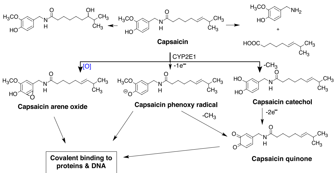
Fig. 4. Proposed bioactivation of capsaicin.
