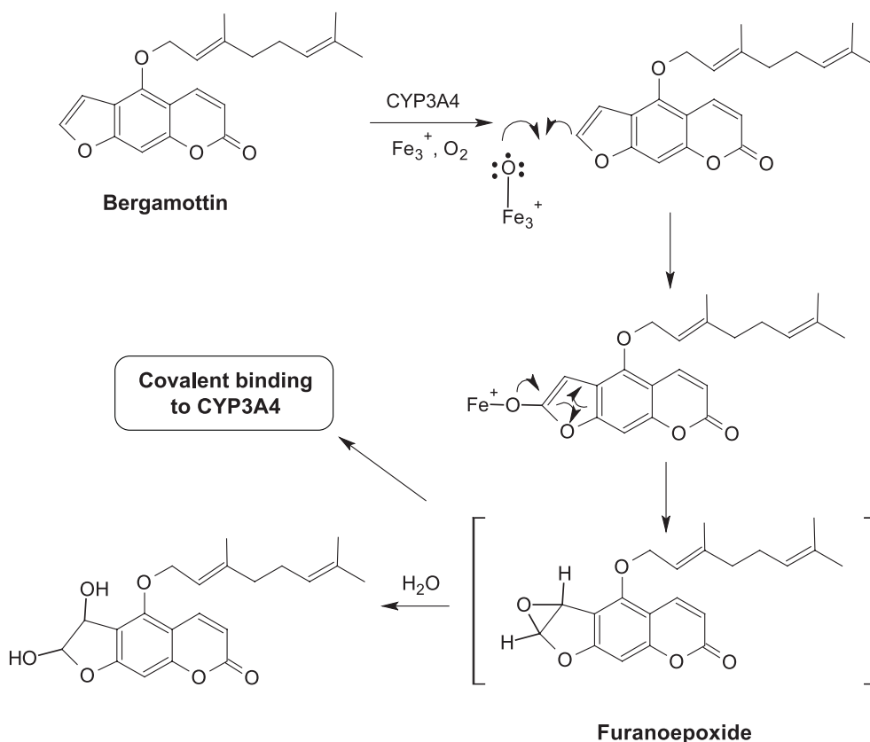
Fig. 5. Proposed bioactivation of bergamottin.
