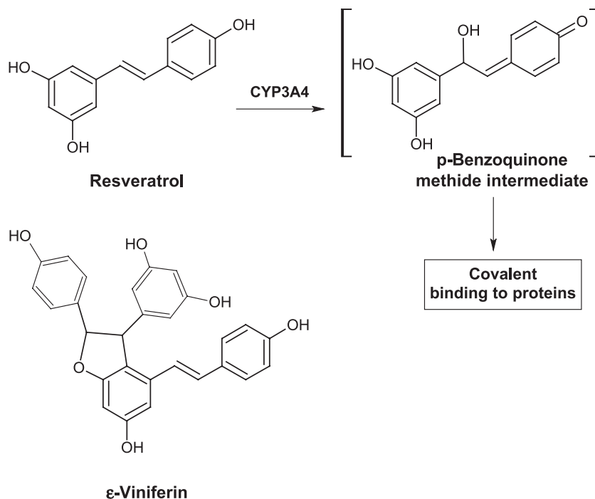
Fig. 12. Proposed bioactivation of resveratrol.
