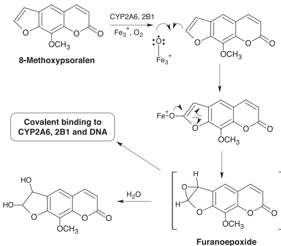
Fig. 6. Proposed bioactivation of 8-methoxypsoralen.
