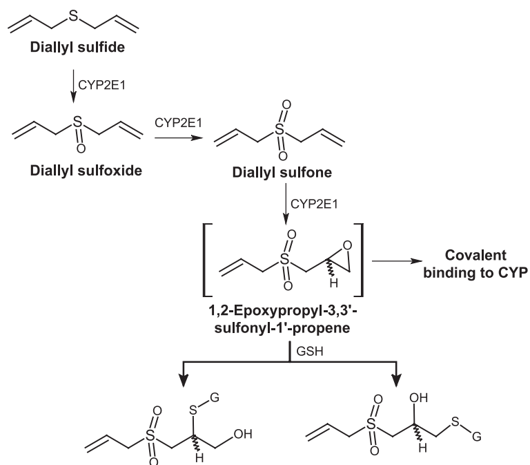
Fig. 11. Metabolism of diallyl sulfide by CYP2E1.
