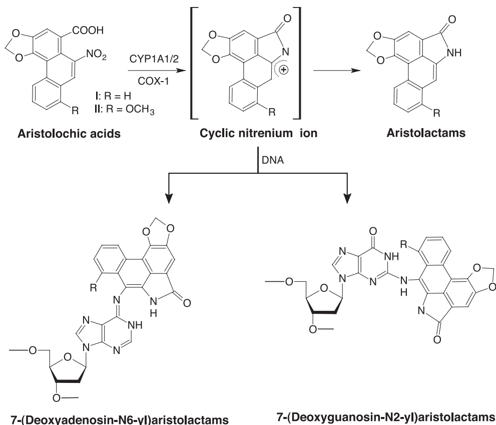
Fig. 1. Proposed bioactivation of aristolochic acids.
