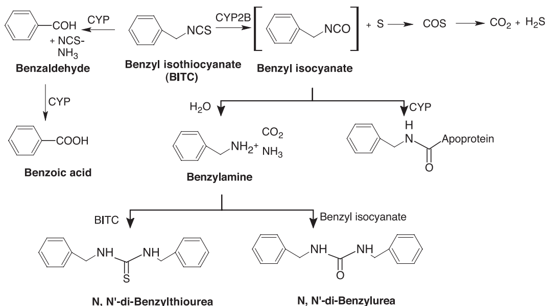
Fig. 8. Proposed bioactivation of benzyl isothiocyanate (BITC).
