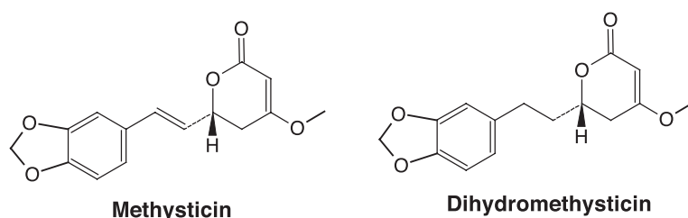
Fig. 9. Chemical structures of methysticin and dihydromethysticin from kava.
