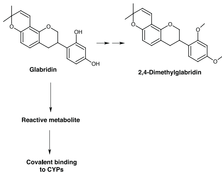
Fig. 7. Chemical structure of glabridin.
