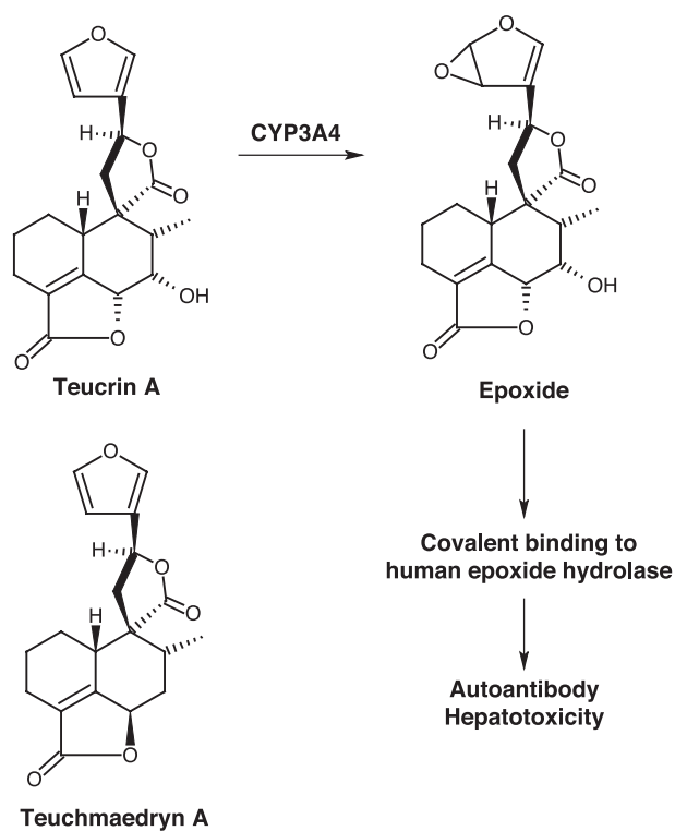
Fig. 3. Proposed bioactivation of teucrin A from germander.
