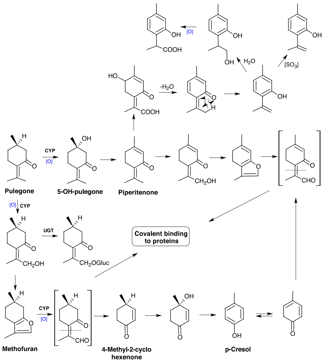
Fig. 2. Proposed bioactivation of pulegone.
