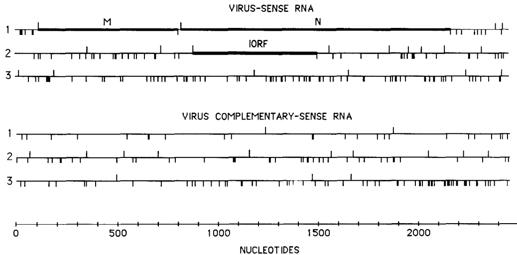
FIG. 3. Schematic diagram of open reading frames obtained when translating the 3' 2451-base sequence of the BCV genome as either virus-sense RNA or virus complementary-sense RNA. Vertical bars above the line represent the first methionine codon that could serve as the initiation site for translation. Vertical bars below the line represent termination codons. M: sequence of the matrix protein gene. N: sequence of the nucleocapsid protein gene. IORF: sequence of an internal open reading frame within the N gene. 5' to 3' orientation is always left to right.
