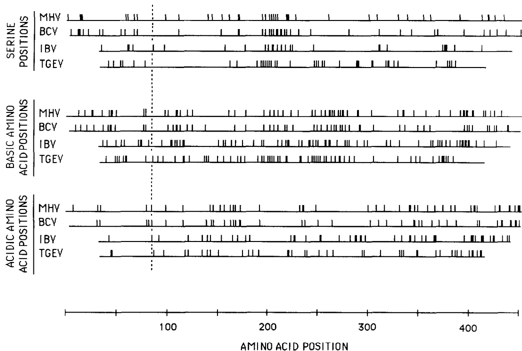
Fig. 6. Positions of serine residues, basic amino acids, and acidic amino acids on the N protein of MHV (A59), BCV (Mebus), IBV (Beaudette), and TGEV (Purdue), depicted in a way to show clustering. The amino terminus is positioned on the left and the proteins (depicted with no gaps in their sequence) are aligned by the first amino acid in the 68-amino-acid region of high homology which is indicated by the stippled line. Amino acid positions are indicated by vertical bars. Proteins are arranged in decreasing order of length.
