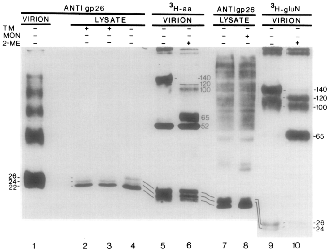
FIG. 5. Identification of different glycosylation states of the M protein. Lane 1: Purified virus immunoblotted with anti-gp26 serum. Lanes 2, 3, and 4: Lysates of infected cells grown respectively in 12, 1.2, or 0 μM tunicamycin (TM), electrophoresed on the same gel as lane 1, and immunoblotted with anti-gp26 serum. Lanes 5 and 6: Purified virus radiolabeled with 3 H-labeled amino acids. Lanes 7 and 8: Lysates of infected cells grown in 0 or 1 μM monensin (MON) and immunoblotted with anti-gp26 serum. Lanes 9 and 10: Purified virus radiolabeled with [ 3 H]glucosamine. Samples treated with 2-mercaptoethanol are indicated (2-ME). The polyacrylamide concentrations are 9% for lanes 1 through 4, and 8% for lanes 5 through 10.
