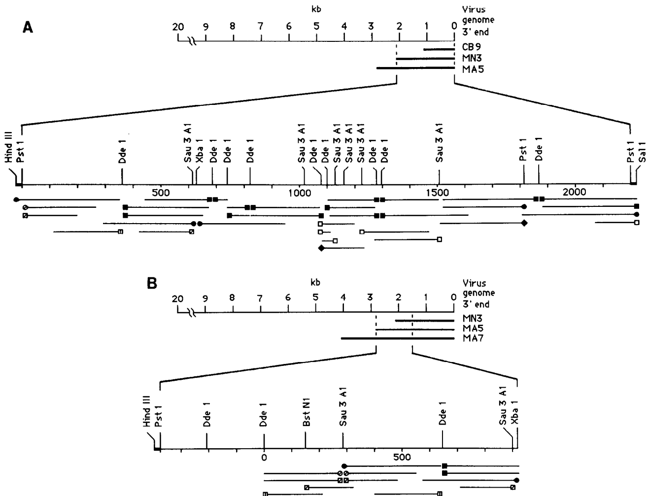
Fig. 1. Sequencing strategy used to obtain BCV genomic sequences containing the N and M genes. (A) Strategy for obtaining the N gene sequence. Clone MN3 was sequenced completely and clones CB9 and MA5 were sequenced in part. The internal Dde I, Pst I, Sau 3A 1, and Xba I sites derived by restriction endonuclease mapping and the Hind III and Sal I sites in the multiple cloning region of the pUC9 vector were the sites used for DNA sequencing. ■, □ and ◻ indicate sites labeled at the 5' end using polynucleotide kinase for clones MN3, CB9, and MA5, respectively. ●, ○, and ◊ indicate sites labeled at the 3' end using reverse transcriptase, and the appropriate labeled deoxynucleotide triphosphate, for clones MN3, CB9, and MA5, respectively. ◆ indicates sites labeled at the 3' end using radiolabeled cordycepin and terminal transferase for a subclone of MN3. (B) Strategy for obtaining the M gene sequence. Parts of clones MN3, MA5, and MA7 were sequenced beginning with the second Dde I site from the 5' end of clone MA5. ■, ◻, and ◻ indicate restriction sites that are 5' end labeled with polynucleotide kinase for clones MN3, MA5, and MA7, respectively. ● and ◊ indicate sites that were 3' end labeled using reverse transcriptase and the appropriate labeled deoxynucleotide triphosphate for clones MN3 and MA5, respectively. Uniquely labeled molecules for sequencing were obtained from gels after electrophoretic separation of restriction endonuclease-treated, end-labeled fragments or after strand separation. The orientation of the clones in the pUC9 vector are as shown except for CB9 which is inverted; i.e., the poly(A) end is next to the Hind III site of the vector. pUC9 sequences are indicated as a bold line at the end of the restriction endonuclease maps.
