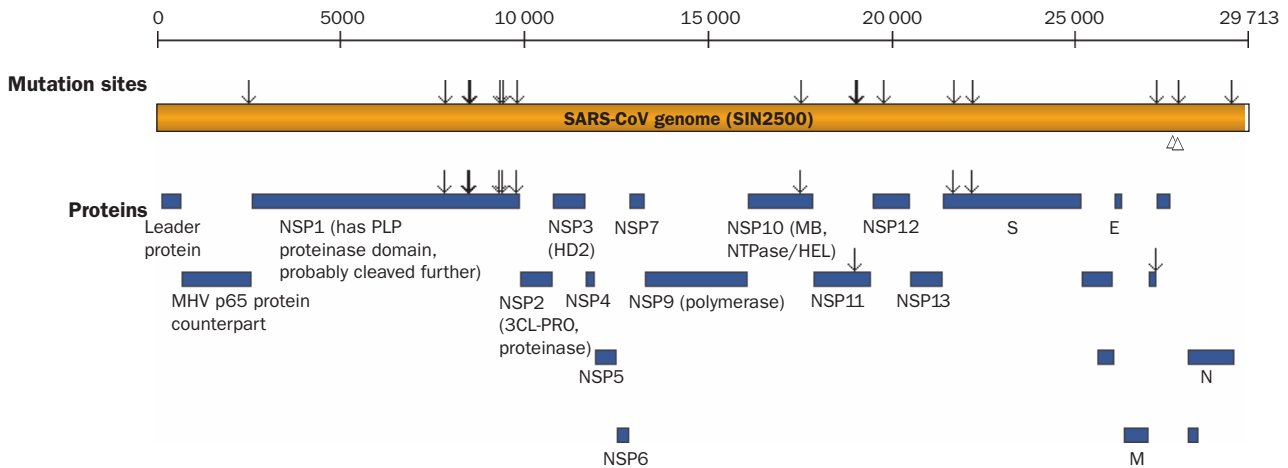
Figure 1: Genome structure of SARS-CoV
