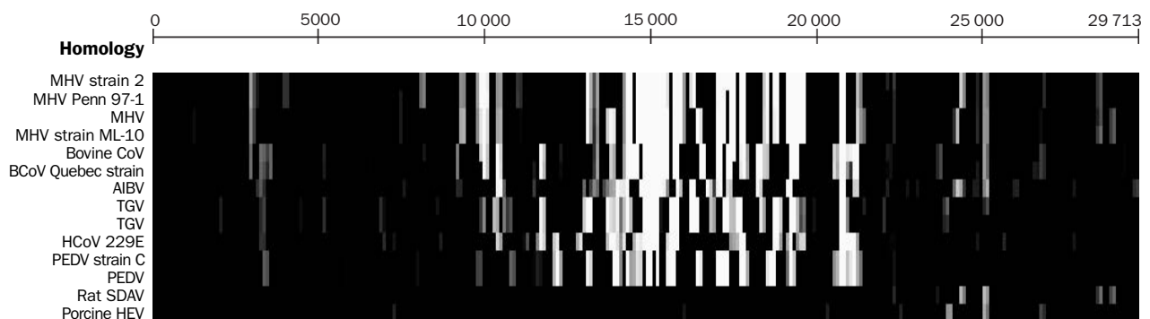
Figure 2: Homology of SARS-CoV genome sequence (SIN2500) to other coronaviruses
