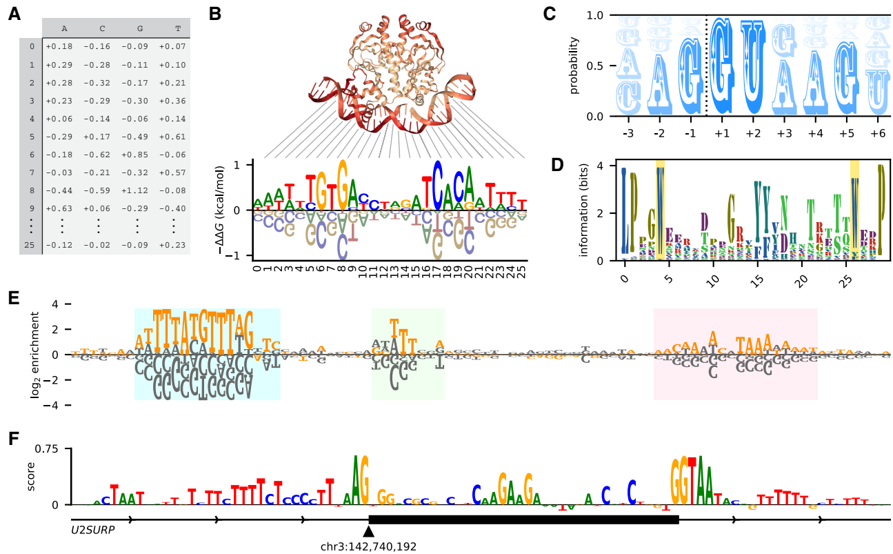
Fig. 1. Logomaker logos can represent diverse types of data. (A) Example input to Logomaker. Shown is an energy matrix for the transcription factor CRP; the elements of this pandas DataFrame represent -\Delta\Delta G values contributed by each possible base (columns) at each nucleotide position (rows). Data are from Kinney et al. (2010). (B) An energy logo for CRP created by passing the DataFrame in panel A to Logomaker. The structural context of each nucleotide position is indicated [PDB 1CGP (Parkinson et al. , 1996)]. (C) A probability logo computed from all annotated 5' splice sites in the human genome (Frankish et al. , 2019). The dashed line indicates the exon/intron boundary. (D) An information logo computed from a multiple alignment of WW domain sequences [PFAM RP15 (Finn et al. , 2014)], with the eponymous positions of this domain highlighted. (E) An enrichment logo representing the effects of mutations within the ARS1 replication origin of S.cerevisiae . Orange characters indicate the ARS1 wild-type sequence; highlighted regions correspond (from left to right) to the A, B1 and B2 elements of this sequence (Rao and Stillman, 1995). Data (unpublished; collected by J.B.K.) are from a mutARS-seq experiment analogous to the one reported by Liachko et al. (2013). (F) A masked logo (Shrikumar et al. , 2017) representing the importance scores of nucleotides in the vicinity of U2SURP exon 9, as predicted by a deep neural network model of splice site selection. Logo adapted (with permission) from Fig. 1D of Jaganathan et al. (2019). The script used to make this figure is posted on the Logomaker GitHub page at logomaker/examples/figure.ipynb
