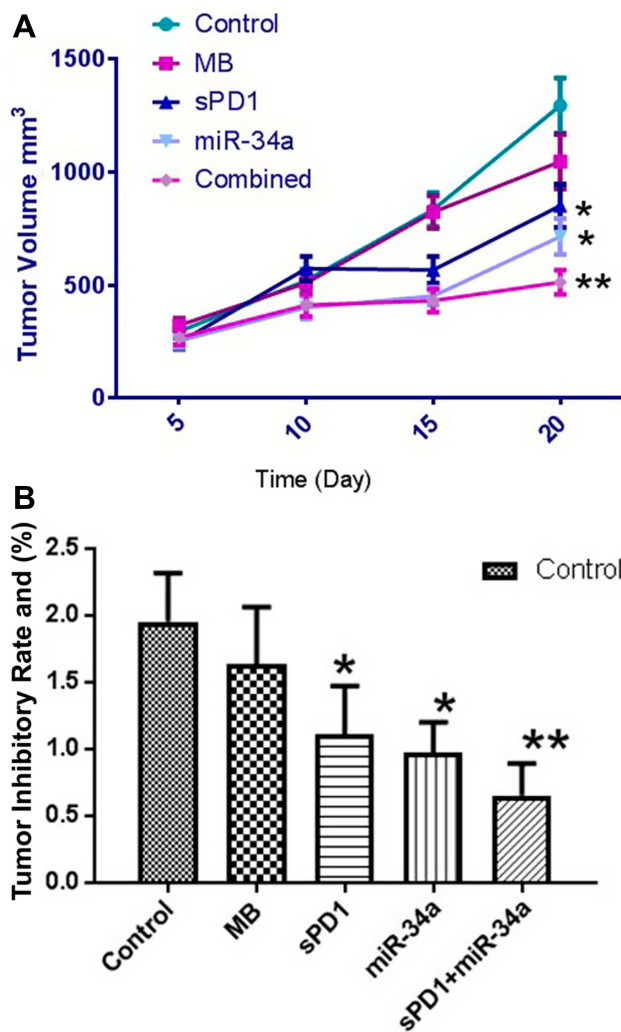
Figure 2 Tumor volume (A) and tumor weight (B) in each group. *P≤0.05. **P≤0.01.
