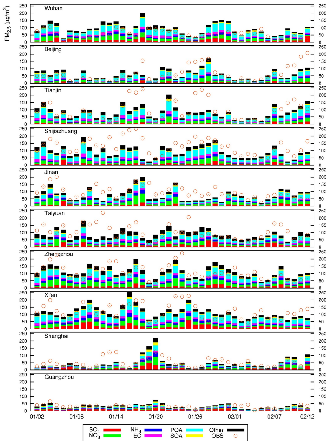
Fig. 2. Predicted daily PM 2.5 and its components with observed daily PM 2.5 in 10 major cities in Case 3. Units are µg/m 3 .
