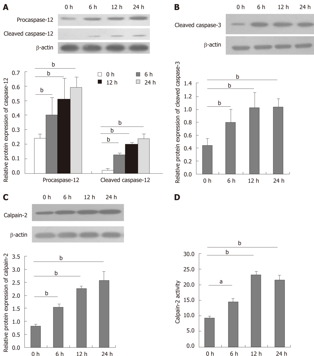
Figure 3 Dithiothreitol induces caspase-12 and caspase-3 activation and increases calpain-2 activity in BRL-3A cells. After treatment with 2.0 mmol/L dithiothreitol for varying periods, the relative levels of caspase-12, cleaved caspase-12 and cleaved caspase-3 as well as calpain-2 expression in each group of BRL-3A cells were quantified by Western blotting. Furthermore, the activity of calpain-2 in each group of cells was measured. Data are representative images or expressed as the mean \pm SD of each group of cells from three separate experiments. A: Caspase-12 activation; B: Caspase-3 activation; C: Calpain-2 expression; D: Calpain-2 activity. a P < 0.05 , b P < 0.01 .
