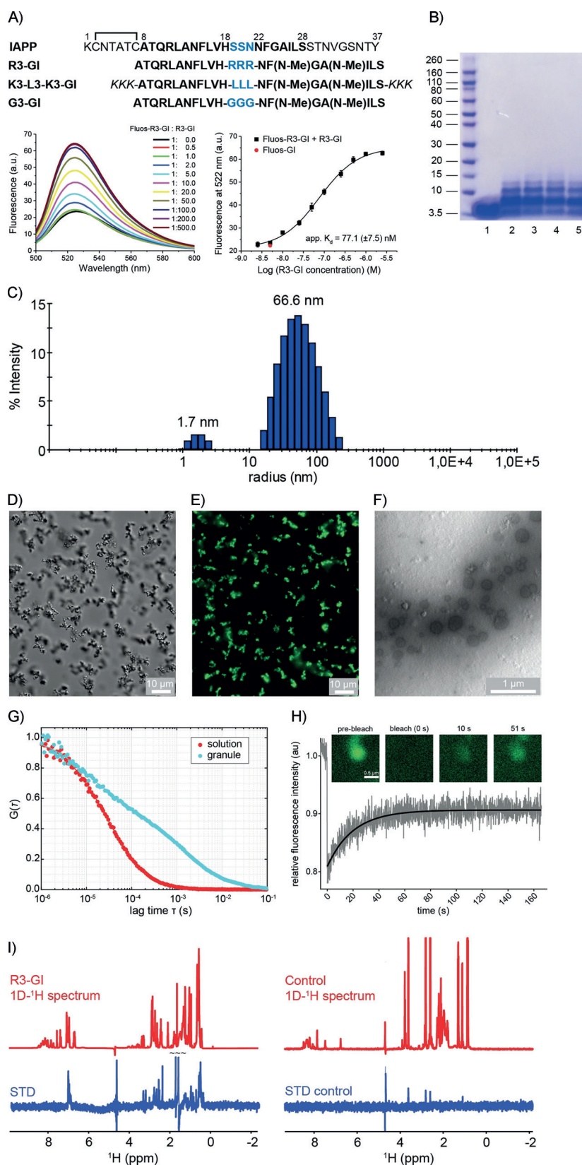
Figure 1. R3-GI self-assembly. A) Top: sequences and abbreviations of IAPP and the investigated ISMs. “Hot segments” of the IAPP interaction surface with A \beta 40 are shown with black bold letters; residues in the IAPP loop and ISM linker regions are drawn in blue. The L3-GI solubilizing tag “KKK” is shown in italics. Bottom: fluorescence emission spectra of N-terminal fluorescein-labeled R3-GI (Fluos-R3-GI; 5 nM) alone and after titration with R3-GI at the indicated molar ratios (pH 7.4). On the right, the binding curve is shown. The estimated app. K_d value for R3-GI self-association is 77.1 ( \pm 7.5) nM. Data are means ( \pm SEM) from three binding curves. B) R3-GI oligomerization (500 \mu M) studied by cross-linking with glutaraldehyde and NuPAGE. Lane 1: R3-GI without cross-linking; lanes 2–5: R3-GI cross-linked following incubation for 0 h (lane 2), 1 h (lane 3), 24 h (lane 4), and 48 h (lane 5). C) DLS studies of a 50 \mu M R3-GI in 10 mM sodium phosphate buffer, pH 7.4 (containing 1% v/v HFIP). D) Differential interference contrast (DIC) micrograph of R3-GI (500 \mu M). The peptide was imaged immediately after dissolution into 10 mM sodium phosphate buffer, pH 7.4 (containing 1% v/v HFIP) without filtration. Scale bar: 10 \mu m. E) Microscopy image of Fluos-R3-GI in fluorescence mode. F) TEM image of R3-GI (500 \mu M) in 10 mM sodium phosphate buffer, pH 7.4 (containing 1% v/v HFIP). Spherical assemblies were observed with diameters in the range of 200–400 nm. G) Fluorescence correlation spectroscopy (FCS) of a mixture of 454 \mu M R3-GI and 454 nM Fluos-R3-GI showing that the translational diffusion inside the R3-GI granules is strongly retarded. H) Fluorescence recovery after photobleaching (FRAP) of a R3-GI granule. The fast recovery of the fluorescence intensity indicates that the majority of the peptide molecules are exchanging with the bulk solution within seconds. I) Saturation transfer difference (STD) NMR experiments of 1.25 mM R3-GI in 10 mM sodium phosphate buffer, pH 7.4 (containing 1% v/v HFIP and 10% v/v D 2 O), showing that soluble, monomeric R3-GI undergoes exchange with a high-molecular-weight oligomeric R3-GI conformer. As a control, STD spectra of a 60 \mu M solution of the peptide GVAE-PEQDCAVTSGE ( M_r = 1.492 kDa) are shown. The control peptide is monomeric under the conditions employed in the experiment.
