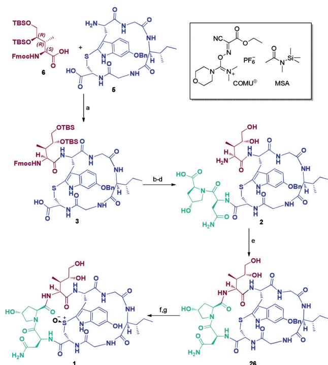
Scheme 5. Fragment couplings and cyclizations to the target molecule \alpha -Amanitin (1): a) MSA, COMU, DIPEA, DMA, 0°C to r.t. 3 h; b) (a and b: onepot), H-Asn-Hyp-OFm-HCl (4), HATU, DIPEA, DMF, 0°C to r.t., 2 h; c) Et 2 NH, DMF, 1 h, r.t.; d) 1 M TBAF, THF, r.t., 2 h, 77% over four steps; e) HATU, DIPEA, DMF, r.t., 16 h, 68%, f) BF 3 ·OEt 2 , EtSH, r.t., 2 h; g) mCPBA, iPrOH/EtOH (2:1), r.t., 30 min, 35% over two steps.
