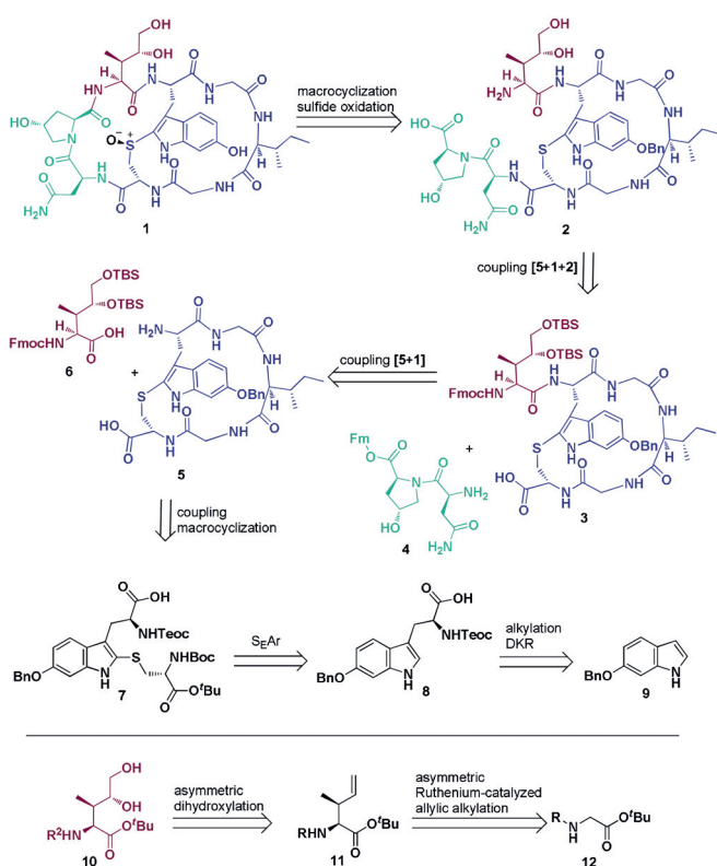
Scheme 1. Retrosynthetic analysis of \alpha -amanitin ( 1 ). Final assembly of \alpha -amanitin from three building blocks and enantioselective synthesis of the hydroxylated amino acid building blocks.
