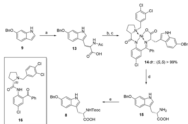
Scheme 2. Synthesis of N -Teoc-6-benzyloxy-L-tryptophan ( 8 ) by dynamic kinetic resolution: a) L-serine, Ac 2 O, AcOH, 75 °C, 2 h, 82%; b) 40% NaOH, MeOH/H 2 O, c) chiral ligand 16 , Ni(NO 3 ) 2 ·6H 2 O, MeOH, reflux, 16 h, 84% over two steps, d) 6 M HCl, MeOH, 70 °C, 2 h, e) TeocOSu, Et 3 N, DMF, 60 °C, 4 d, quant.
