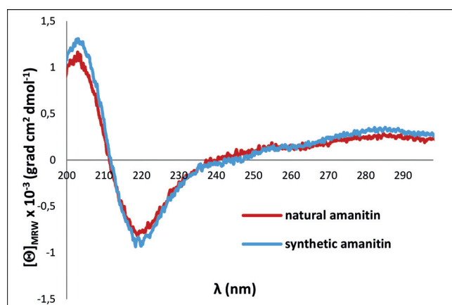
Figure 2. CD spectra of natural and synthetic \alpha -amanitin (1).
