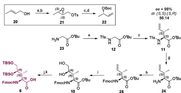
Scheme 4. Synthesis of side chain-protected Fmoc-(3 R ,4 R )-4,5- L -dihydroxyisoleucine ( 6 ) a) (+)-DIPT, \text{Ti}(\text{O}i\text{Pr})_4 , TBHP, DCM, -20^\circ\text{C} , 4 h; b) TsCl, \text{Et}_3\text{N} , DMAP, DCM, -10^\circ\text{C} , 30 h, 67%; c) NaI, Zn(Cu), THF, 70^\circ\text{C} , 2 h; d) \text{Boc}_2\text{O} , NaH, THF, 0^\circ\text{C} to r.t., 16 h, 75%; e) ethyl trifluoroacetate, \text{NET}_3 , MeOH, r.t., 16 h, quant.; f) LHMDS, \text{ZnCl}_2 , \text{PPh}_3 , [( p -cymene) \text{RuCl}_2 ] 2 , 22 , THF, -72^\circ\text{C} to r.t., 16 h, 88%; g) \text{NaBH}_4 , MeOH, r.t., 1 h; h) FmocOSu, \text{Et}_3\text{N} , dioxane, r.t., 4 h, 82%; i) \text{K}_2\text{OsO}_4 \cdot \text{H}_2\text{O} , NMO, \text{CHCl}_3/\text{H}_2\text{O} , r.t., 6 h, 40%; j) TBSCl, pyridine/DMF(1:9), r.t., 24 h, 95%; k) TMSOTf, 2,6-lutidine, 0^\circ\text{C} to r.t., 2 h, 90%.
