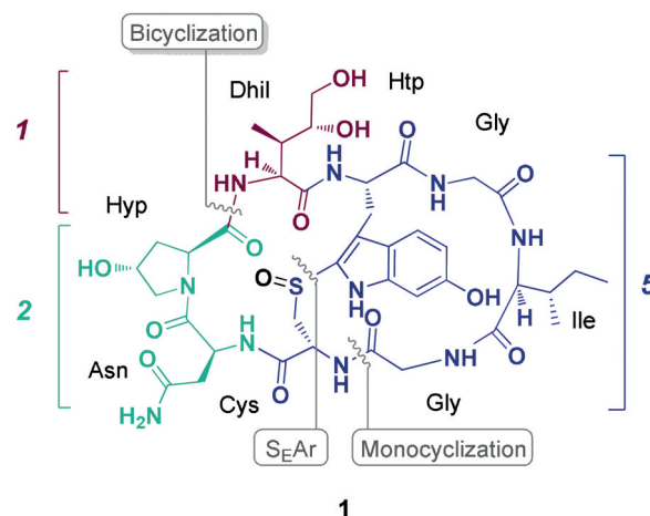
Figure 1. Structure of \alpha -Amanitin ( 1 ). The numbers in blue, turquoise and red refer to the number of amino acids of the building blocks (depicted blue, turquoise and red) employed in this total synthesis strategy [5+1+2].
