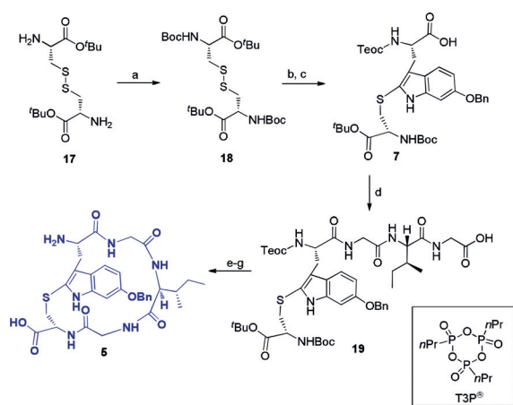
Scheme 3. Synthesis of the C- and N-terminally deprotected monocyclic tryptathionine peptide 5 : a) \text{Boc}_2\text{O} , \text{NaHCO}_3 , dioxane/ \text{H}_2\text{O} , r.t., 16 h, 99%; b) \text{SO}_2\text{Cl}_2 , \text{CHCl}_3 , r.t., 1 h; c) 8 , \text{NaHCO}_3 , \text{CHCl}_3 , 0^\circ\text{C} to r.t., quant.; d) H-Gly-Ile-Gly-OH, \text{CO}(\text{OSu})_2 , collidine, acetonitrile/ \text{H}_2\text{O} , r.t., 2 h; e) PTSA, THF, r.t., 2 h, 70% over 2 steps; f) T3P, DIPEA, DMF, r.t., 16 h, 70%, g) TFA/ \text{H}_2\text{O} (7:3), r.t., 2 h, quant.
