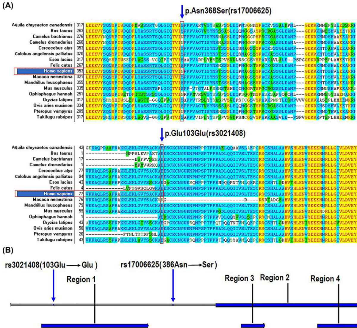
Figure 2. Multiple-sequence alignment and position analysis of rs3021408 and rs17006625 (A) Multiple-sequence alignment of KAT2B from birds, fishes and mammals (including Homo sapiens , Pan troglodytes , Macaca mulatta etc.). (B) Position analysis of the SNPs in the KAT2B protein.
