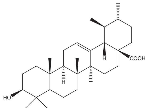
Figure 3 Ursolic acid. [81]
