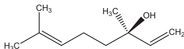
Figure 2 Linalool. [80]
