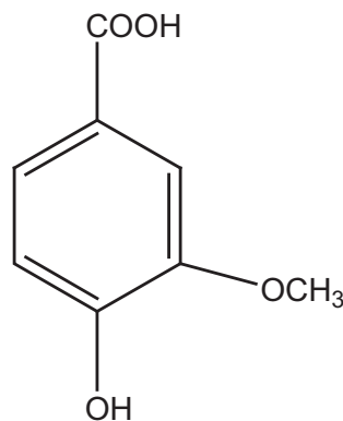
Figure 6 Vanillic acid. [84]
