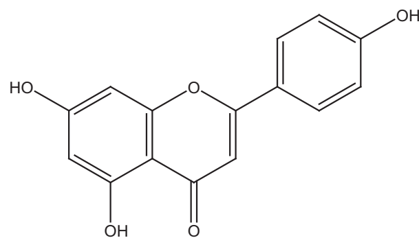
Figure 1 Apigenin. [79]
