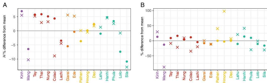
Fig. 2 Diversity statistics shown as the percent difference from the mean. a The haplotype diversity ( H ) and b the nucleotide diversity ( \pi ). Crosses and dots denote the MSY and mtDNA values, respectively. Population labels are color coded by language family with Austro-
