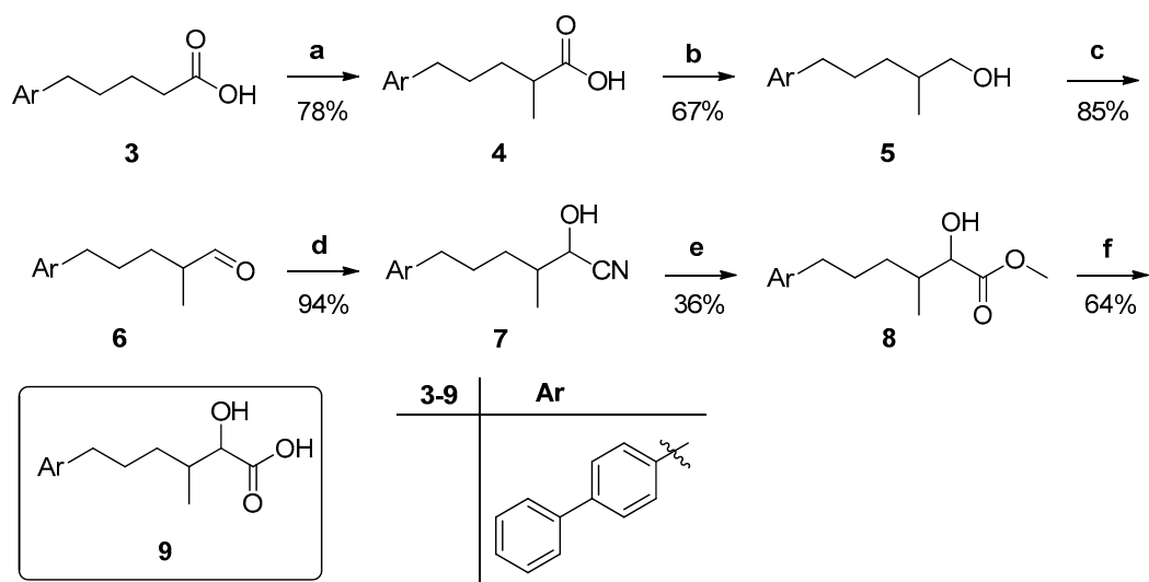
Scheme 1. Synthesis of 2-hydroxy acid 9 . (a) (i) LDA, dry THF (ii) HMPA, (iii) CH 3 I; (b) (i) CH 3 CH 2 OCOC(=O)Cl, Et 3 N, dry THF, (ii) NaBH 4 , MeOH; (c) iodobenzene diacetate, TEMPO (10 mol%), dry CH 2 Cl 2 ; (d) aq. sol. NaHSO 3 , CH 2 Cl 2 , (ii) KCN, H 2 O; (e) 6N HCl/MeOH; (f) 1N NaOH, MeOH.
