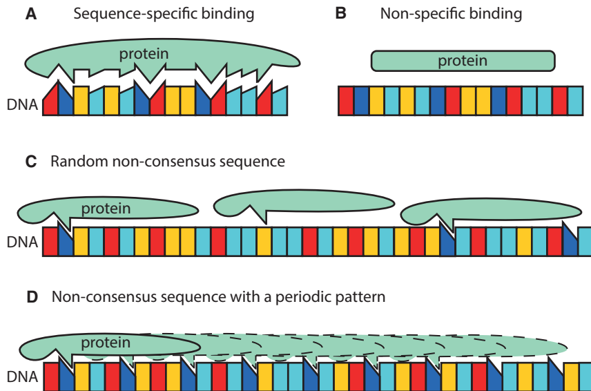
FIGURE 1 Protein-DNA binding is not limited to sequence specific (A) and nonspecific (B). It can also be characterized by an intermediate regime of nonconsensus binding, which is nonspecific for random DNA sequences (C) but has an increased binding strength for DNA regions enriched with certain repeated nucleotide patterns (D). The DNA lattice units shown in different colors may correspond to individual basepairs or larger regions. Different geometric shapes of such units used on the figure do not imply that such shapes are actually visible in the DNA structure—these may also correspond to alterations of the DNA double helix stability or other slight perturbations of the energy landscape. To see this figure in color, go online.
