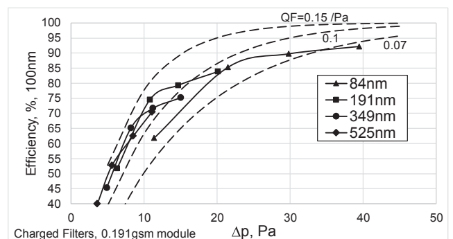
Fig. 7. Efficiency of 100-nm aerosol versus pressure drop for electret multilayer versus single layer for 84 nm, 191 nm, and 525 nm diameter filters. Iso-QF curves for 0.07, 0.1 and 0.15 Pa -1 are shown.
