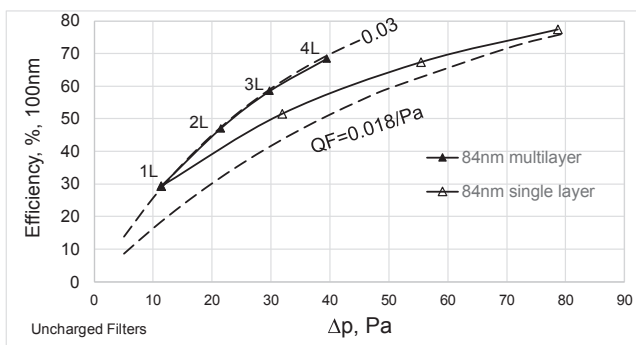
Fig. 6a. Efficiency of nano-aerosols versus pressure drop for multilayer versus single layer for 84-nm diameter filter. Iso-QF curves for 0.018 and 0.03 Pa -1 are shown.
