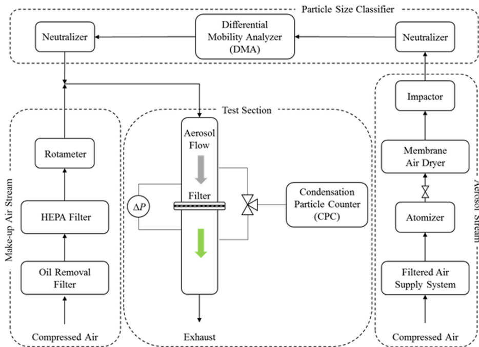
Fig. 1c. Aerosol generator and filter tester.
