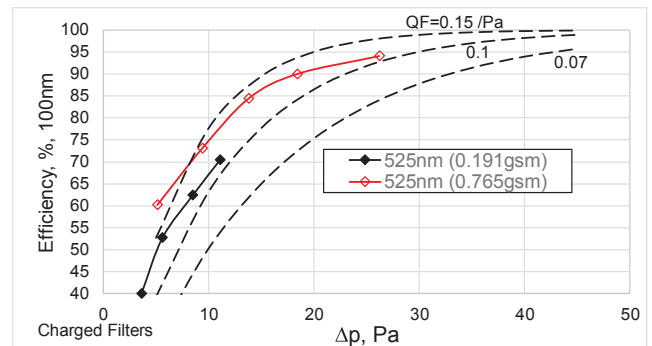
Fig. 9a. Comparing multi-layered filters at 525 nm diameter with modules, respectively, 0.191 gsm and 0.764 gsm.
