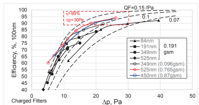
Fig. 9b. Larger diameter nanofiber (450 nm and 525 nm) with increased basis weight (0.87 and 0.765 gsm) were used as basic module for building multilayer filter. These followed the iso-QF curves initially and have some deviations for the 3rd and 4th modules in the multilayer filter.
