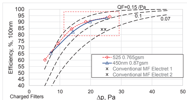
Fig. 10. Comparing the optimized multilayer nanofiber electret filter with conventional microfiber electret.
