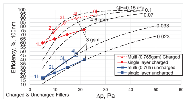
Fig. 11b. Electret/charged versus uncharged (mechanical) filters, and multi-layer versus single-layer filters all with 525-nm fiber diameter (3.06–4.6 gsm filter).
