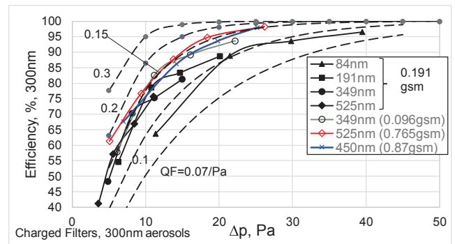
Fig. 12. Efficiency based on 300 nm for 7 multilayer nanofiber electret filters.
