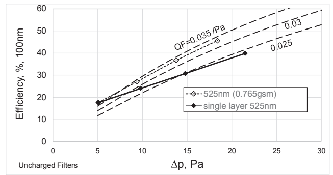
Fig. 6b. Efficiency of 100 nm versus pressure drop for discharged (mechanical) multilayer versus single layer for 525-nm diameter filter. Iso-QF curves for 0.025, 0.03 and 0.035 Pa -1 are shown.
