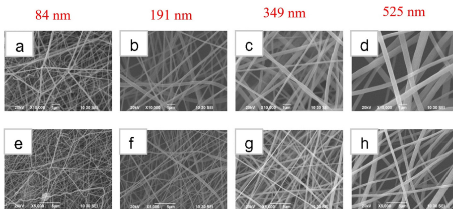
Fig. 2. SEM images of four different electrospun nanofiber diameters in zoom-in view (see 1- \mu\text{m} bar) and zoom-out view (see 5- \mu\text{m} bar). (a) and (e) Correspond to 84 nm, (b) and (f) 191 nm, (c) and (g) 349 nm, and (d) and (h) 525 nm.
