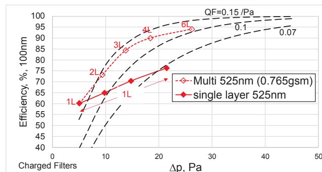
Fig. 11a. Multilayer versus single layer for 525-nm diameter charged filter.
