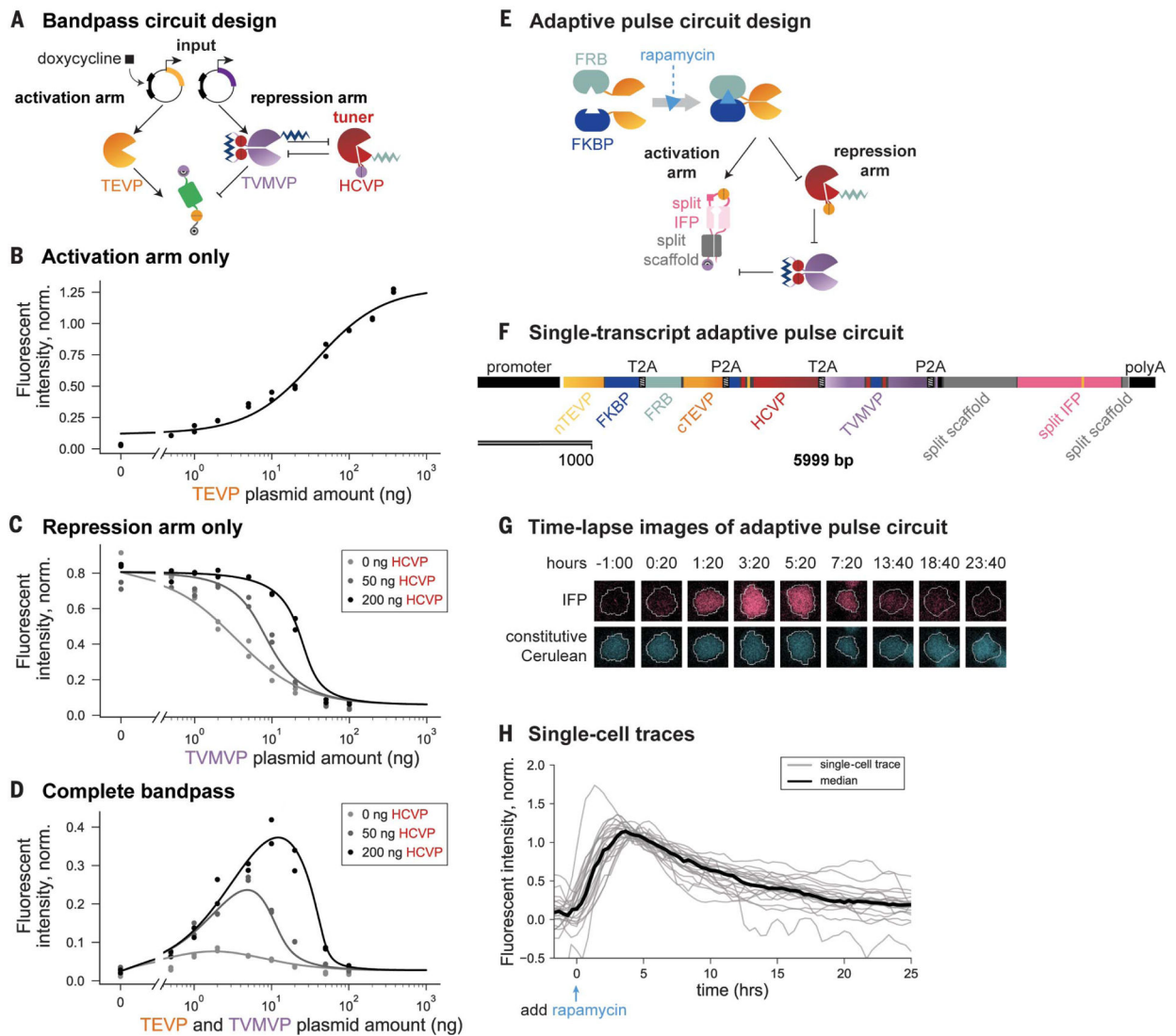
Fig. 3. Design of bandpass filtering and pulse-generation circuits.
