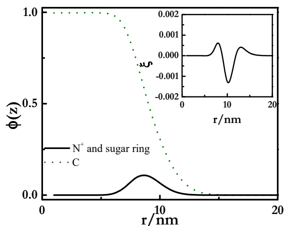
Figure 9. Radial volume fraction, \phi(z) , profiles for the inner hydrophobic core and the charged corona of PDADMAC-di-RL complexes. The polyelectrolyte had a length of 100 segments and a segment valence \nu_p = 1 . The inset represents the dimensionless radial charge density ( \xi ) profiles for the complexes.
