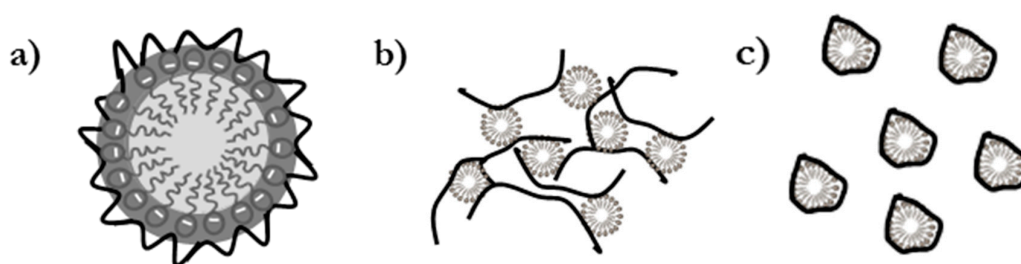
Figure 2. (a) Scheme representing the model assumed for Self-Consistent Mean-Field Calculations (SCF) calculations. (b) Scenario for those systems in which micelles bridge several polymer chains (formation of multichain complexes, g_{PS} > 1 ). (c) Scenario for those systems in which micelles do not bridge polymer chains ( g_{PS} < 1 ).
