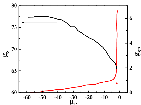
Figure 8. Dependences of the aggregation number of surfactants in the complexes ( g_s , left axis) and the degree of polyelectrolyte-surfactant binding ( g_{PS} , right axis) on \mu_P for mixtures of PDADMAC with di-RL.
