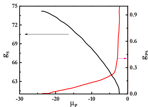
Figure 6. Dependences of the aggregation number of surfactants in the complexes ( g_S , left axis) and the degree of polyelectrolyte-surfactant binding ( g_{PS} , right axis) on \mu_P for mixtures of PDADMAC with APG.
