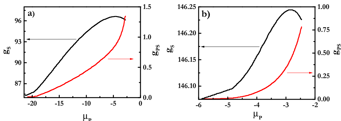
Figure 3. Dependences of the aggregation number of surfactants in the complexes ( g_s , left axis) and the degree of polyelectrolyte-surfactant binding ( g_{PS} , right axis) on \mu_P for mixtures of PDADMAC with SLES (a) and with CB (b).
