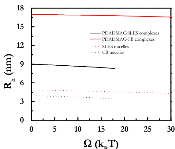
Figure 5. Grand potential \Omega dependences of the hydrodynamic radius, R_h , for the polymer-surfactant complexes and the surfactant micelles in absence of polyelectrolyte.
