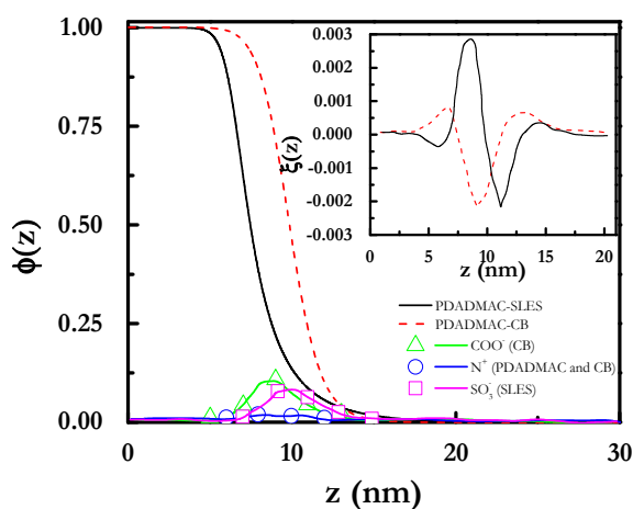
Figure 4. Radial volume fraction ( \varphi(z) ) profiles for the inner hydrophobic core and the charged corona of polyelectrolyte-surfactant complexes. The polyelectrolyte had a length of 100 segments and a segment valence \nu_p = 1 . The inset represents the dimensionless radial charge density ( \xi ) profiles for the complexes.
