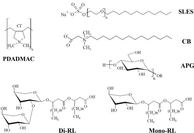
Figure 1. Molecular structures for the polyelectrolyte and the surfactants used in this study, n for SLES assumes a value of 5 and for APG, di-RL, and mono-RL a value of 10.
