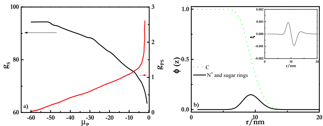
Figure 10. (a) Dependences of the aggregation number of surfactants in the complexes ( g_s , left axis) and the degree of polyelectrolyte–surfactant binding ( g_{PS} , right axis) on the chemical potential of the polymer \mu_p for mixtures of PDADMAC with mono-RL. (b) Radial volume fraction ( \phi(z) ) profiles for the inner hydrophobic core and the charged corona of PDADMAC-mono-RL complexes. The polyelectrolyte had a length of 100 segments and a segment valence \nu_p = 1 . The inset represents the dimensionless radial charge density ( \xi ) profiles for the complexes.
