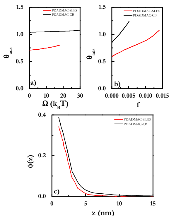
Figure 11. (a) Grand potential ( \Omega ) dependence of the coverage, \theta_{ads} , for different polyelectrolyte–surfactant mixtures. (b) f -ratio, which defines the ratio between the number of monomers and the number of surfactant molecules, dependence of the coverage, \theta_{ads} , dependences for different polyelectrolyte–surfactant mixtures. (c) Volume fraction profiles, \phi(z) , as a function of the distance z from the surface for the different studied mixtures.
