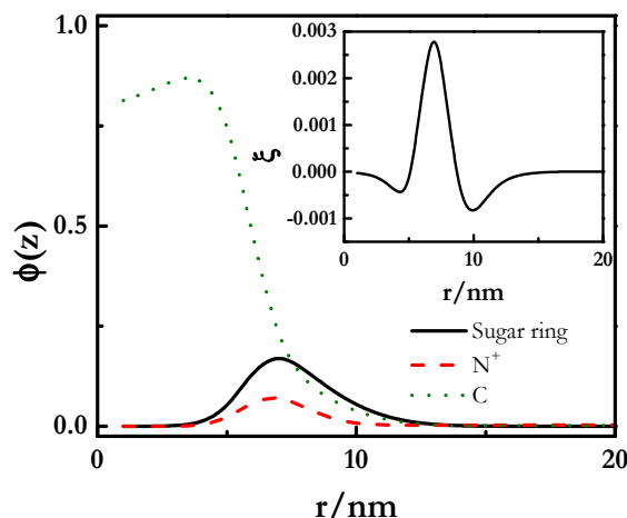
Figure 7. Radial volume fraction ( \varphi(z) ) profiles for the inner hydrophobic core and the charged corona of PDADMAC-APG complexes. The polyelectrolyte had a length of 100 segments and a segment valence \nu_p = 1 . The inset represents the dimensionless radial charge density ( \xi ) profiles for the complexes.
