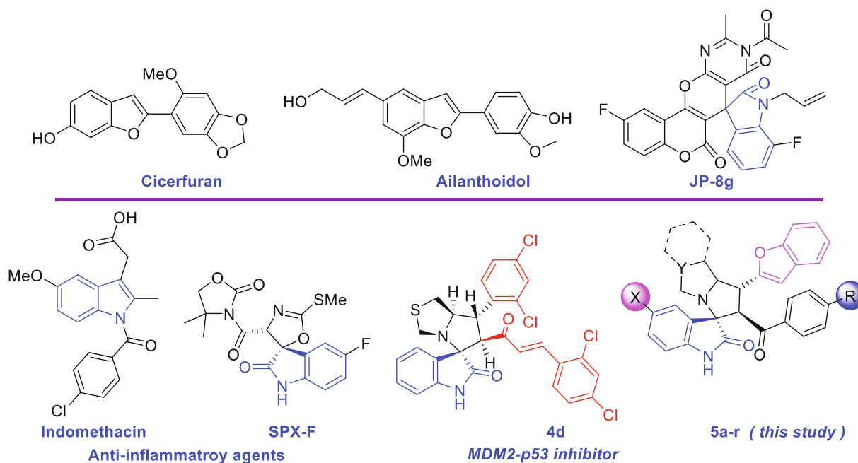
Fig. 1. Representative examples of spirooxindoles and benzo[b]furan scaffolds.
